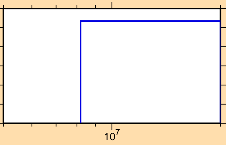
\sigma vs. E for ^{68}\text{Ge}(\text{mt117})
