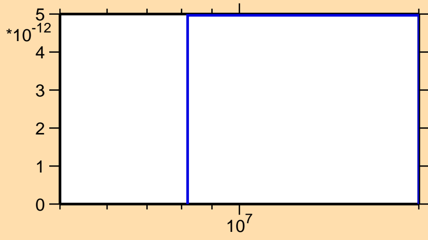
\sigma vs. E for ^{68}\text{Ge}(n,\text{pt})
