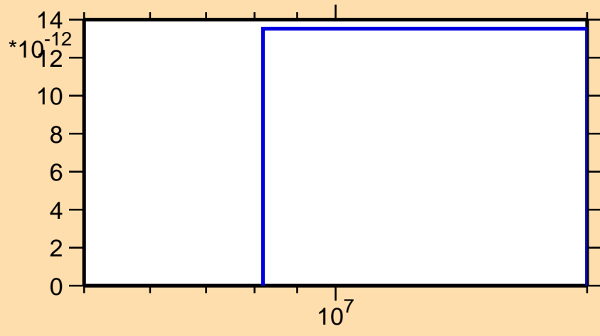
\sigma vs. E for ^{68}\text{Ge}(n,2n\alpha)
