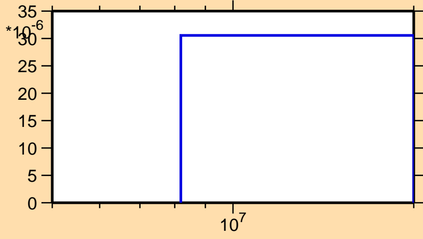
\sigma vs. E for ^{68}\text{Ge}(n,t)
