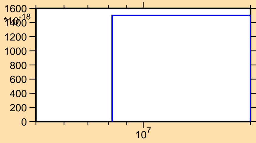
\sigma vs. E for ^{68}\text{Ge} (mt 34)
