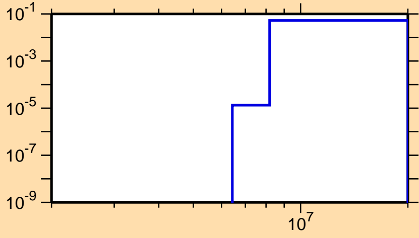
\sigma vs. E for ^{68}\text{Ge}(n,n\alpha)
