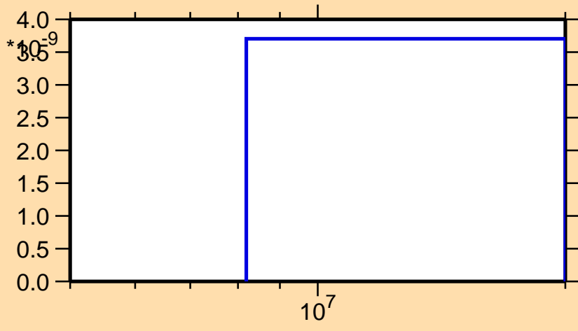
\sigma vs. E for ^{68}\text{Ge} (mt 45)
