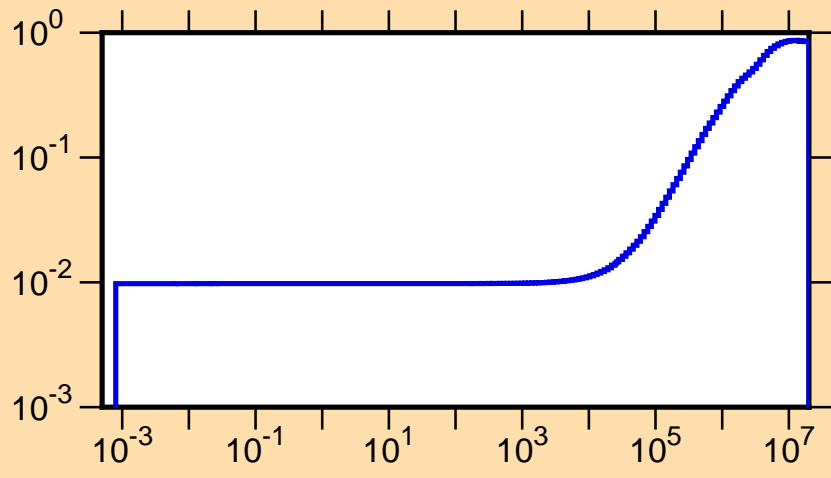
\mu vs. E for ^{69}\text{Ge}(\text{mt251})
