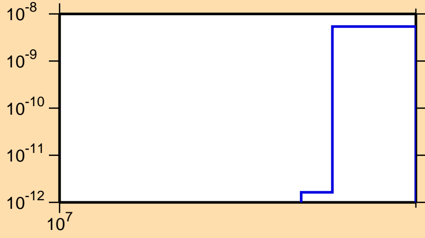
\sigma vs. E for ^{69}\text{Ge} (mt 34)
