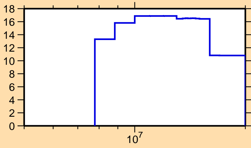
\Delta\sigma/\sigma vs. E for ^{69}\text{Ge}(n,\text{el.})
