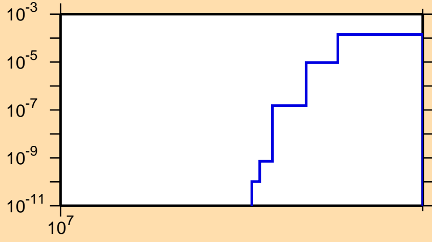
\sigma vs. E for ^{69}\text{Ge}(n,\text{nd})
