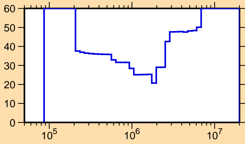
\Delta\sigma/\sigma vs. E for ^{69}\text{Ge}(n,n_1)
