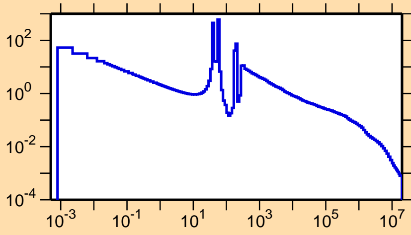
\sigma vs. E for ^{69}\text{Ge}(n,\gamma)
