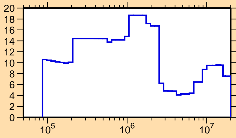
\Delta\sigma/\sigma vs. E for ^{69}\text{Ge}(n,\text{tot.})
