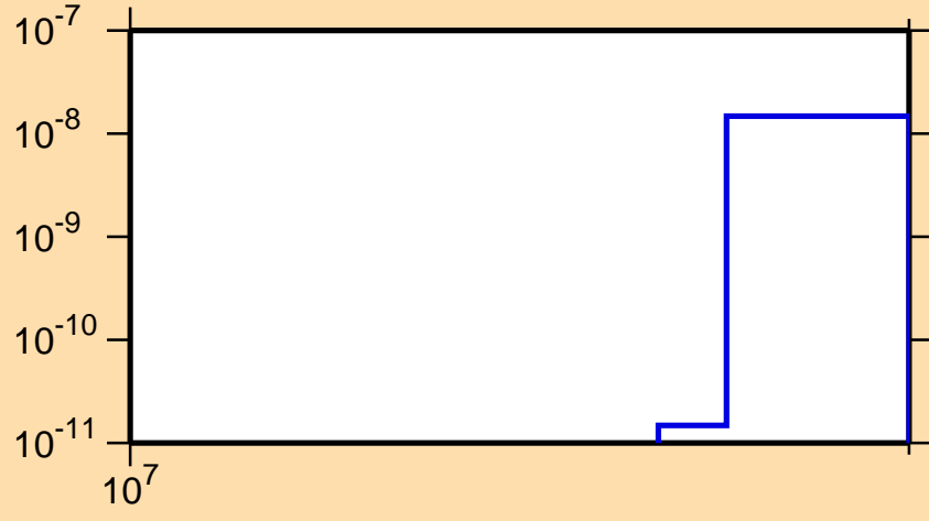
\sigma vs. E for ^{69}\text{Ge} (mt 45)
