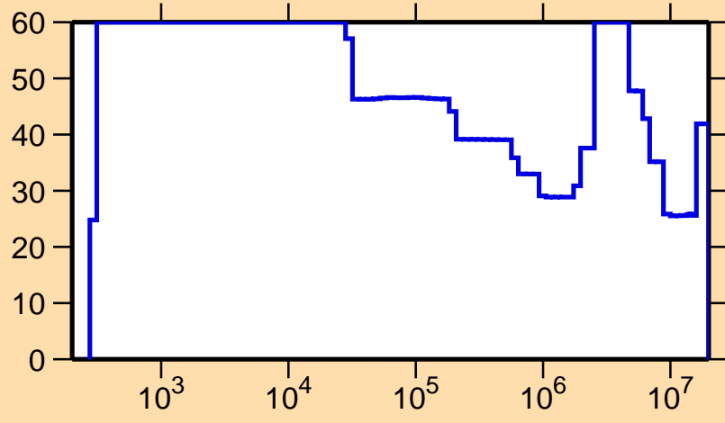
\Delta\sigma/\sigma vs. E for ^{69}\text{Ge}(n,p)
