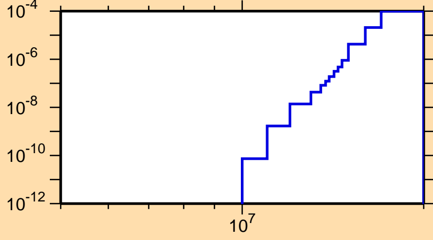
\sigma vs. E for ^{69}\text{Ge}(n,\text{He3})
