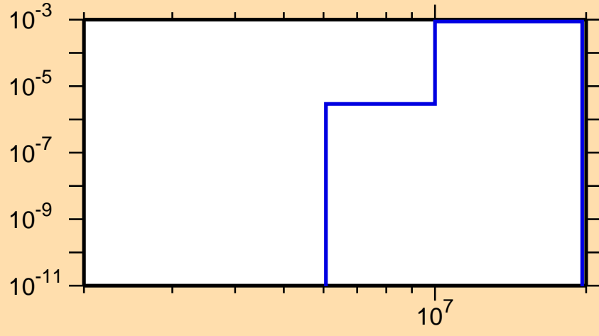
\sigma vs. E for ^{69}\text{Ge}(n,p\alpha)
