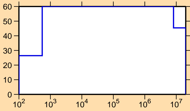
\Delta\sigma/\sigma vs. E for ^{69}\text{Ge}(n,\gamma)
