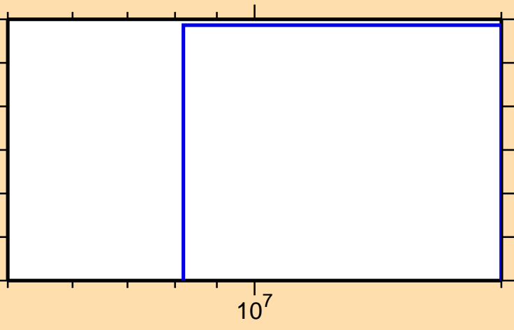
\sigma vs. E for ^{69}\text{Ge}(n,2np)
