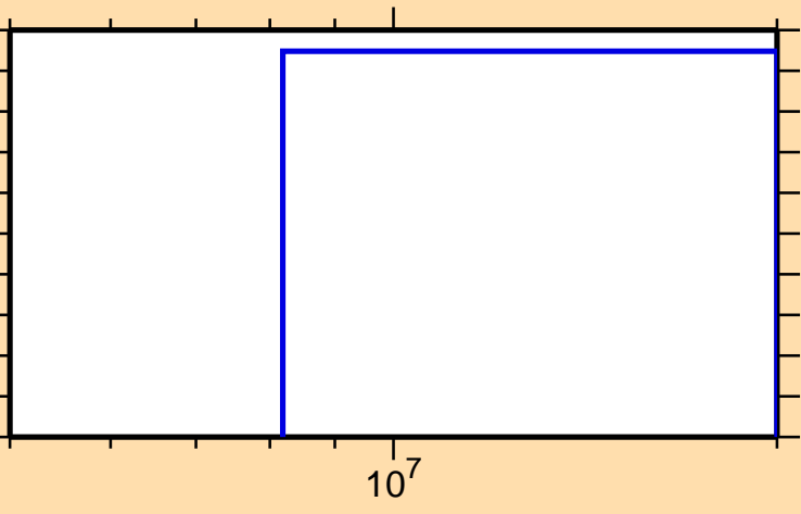
\sigma vs. E for ^{69}\text{Ge}(n,\text{pt})
