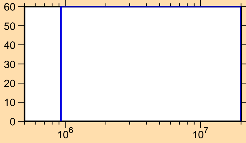
\Delta\sigma/\sigma vs. E for ^{70}\text{Ge}(n,\gamma)
