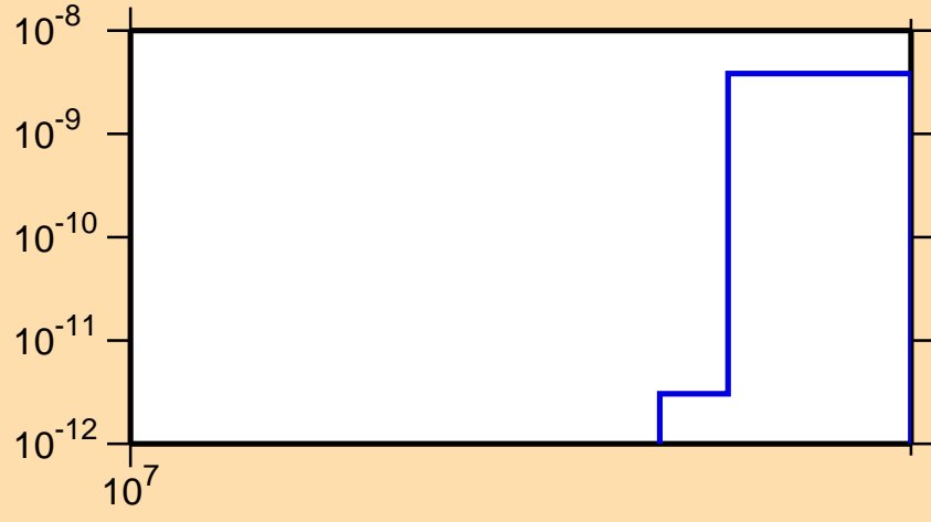
\sigma vs. E for ^{70}\text{Ge} (mt117)
