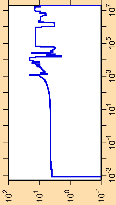
\Delta\sigma/\sigma vs. E for ^{70}\text{Ge}(n,\text{el.})
