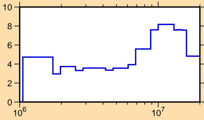
\Delta\sigma/\sigma vs. E for ^{70}\text{Ge}(n,\text{tot.})
