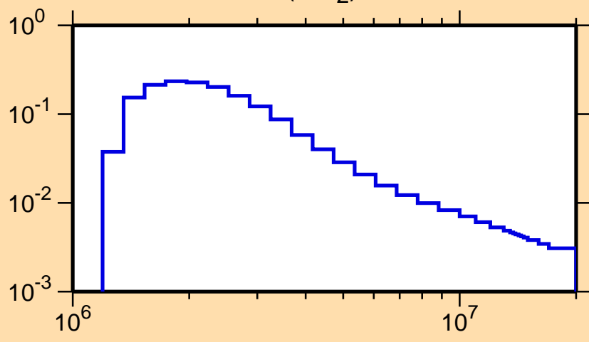
\sigma vs. E for ^{70}\text{Ge}(n,n_2)
