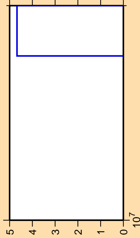
\Delta\sigma/\sigma vs. E for ^{70}\text{Ge}(n,2np)
