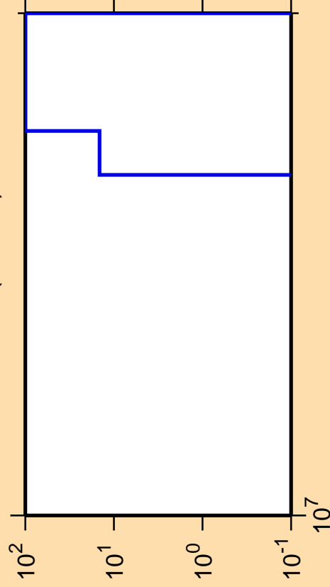
\Delta\sigma/\sigma vs. E for ^{70}\text{Ge} (mt117)
