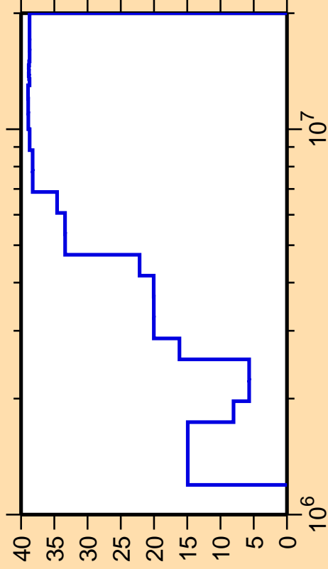
\Delta\sigma/\sigma vs. E for ^{70}\text{Ge}(n,n_2)
