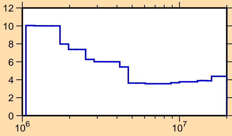
\Delta\sigma/\sigma vs. E for ^{70}\text{Ge}(n,\text{nonel.})
