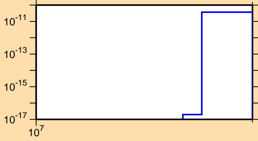
\sigma vs. E for ^{70}\text{Ge} (mt 45)
