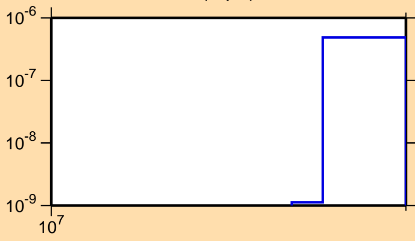
\sigma vs. E for ^{70}\text{Ge}(n,\text{pd})
