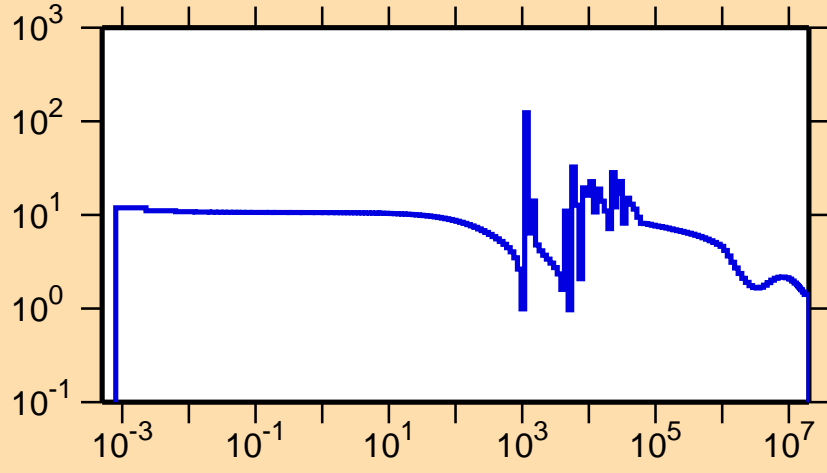
\sigma vs. E for ^{70}\text{Ge}(n,\text{el.})
