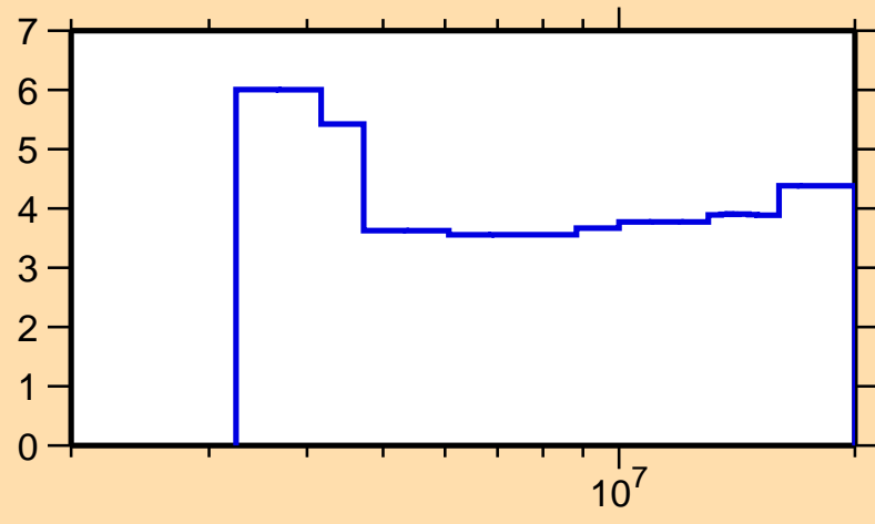
\Delta\sigma/\sigma vs. E for ^{70}\text{Ge}(n,n\text{onel.})
