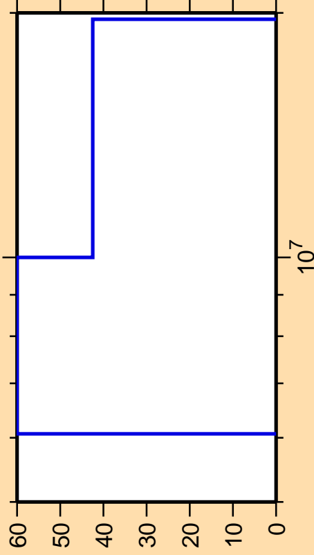
\Delta\sigma/\sigma vs. E for ^{70}\text{Ge}(n,np)
