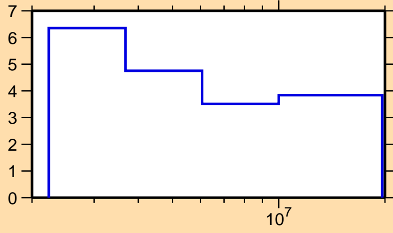
\Delta\sigma/\sigma vs. E for ^{70}\text{Ge}(n,n\text{inel.})
