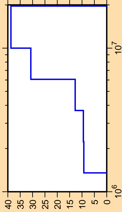
\Delta\sigma/\sigma vs. E for ^{70}\text{Ge}(n,n_3)
