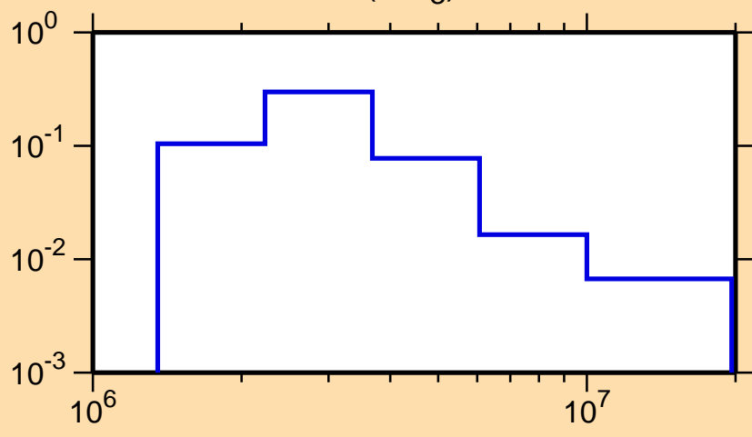
\sigma vs. E for ^{70}\text{Ge}(n,n_3)
