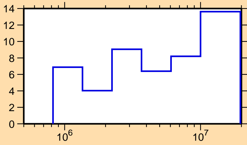
\Delta\sigma/\sigma vs. E for ^{70}\text{Ge}(n,el.)
