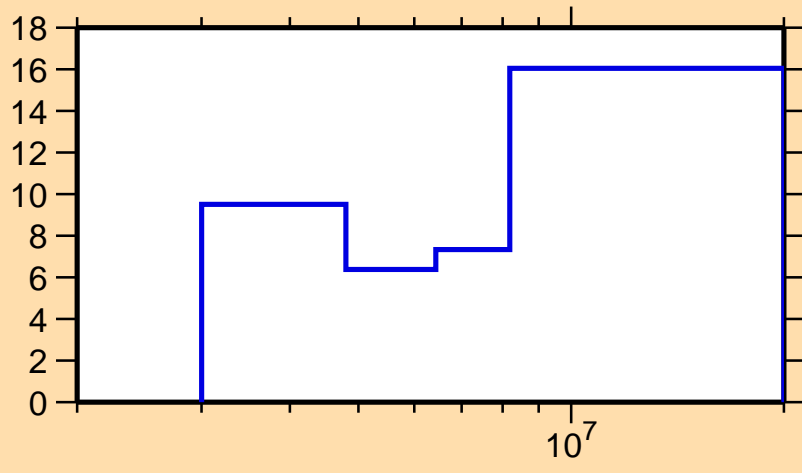
\Delta\sigma/\sigma vs. E for ^{70}\text{Ge}(n,ncont.)
