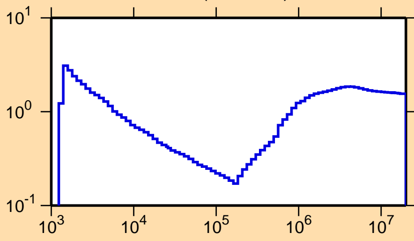
\sigma vs. E for ^{71}\text{Ge}(n,\text{nonel.})
