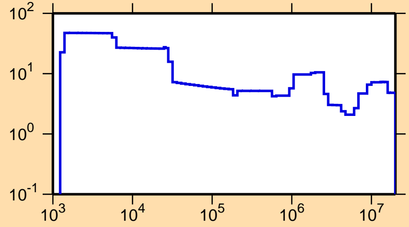
\Delta\sigma/\sigma vs. E for ^{71}\text{Ge}(n,\text{tot.})
