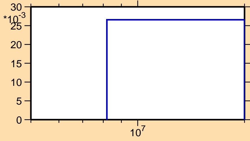
\sigma vs. E for ^{71}\text{Ge}(n,np)
