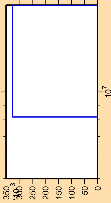
\Delta\sigma/\sigma vs. E for ^{71}\text{Ge} (mt 34)
