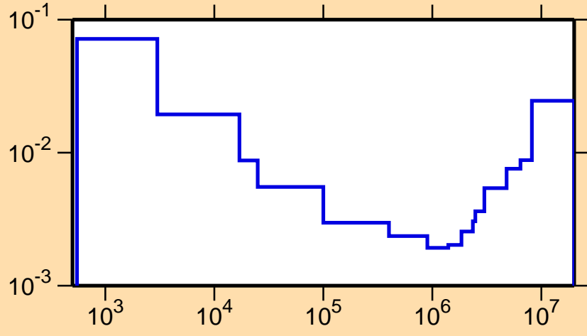
\sigma vs. E for ^{71}\text{Ge}(n,\alpha)
