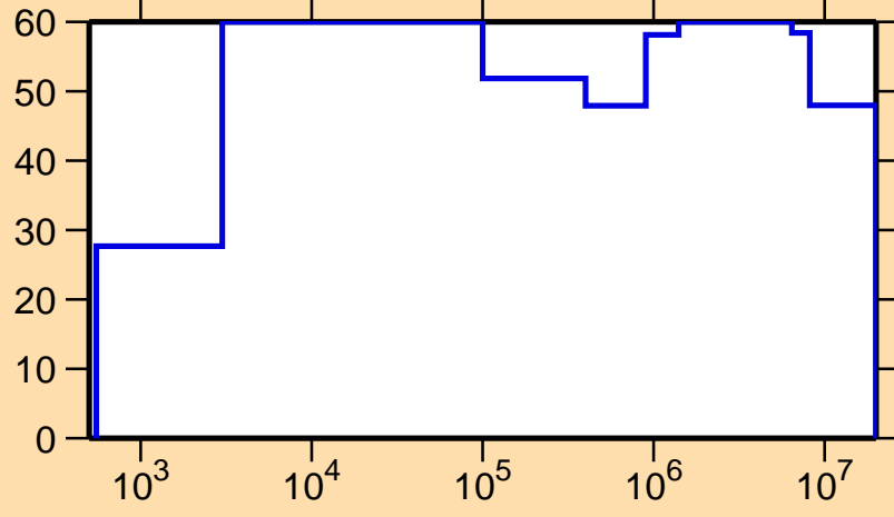
\Delta\sigma/\sigma vs. E for ^{71}\text{Ge}(n,p)
