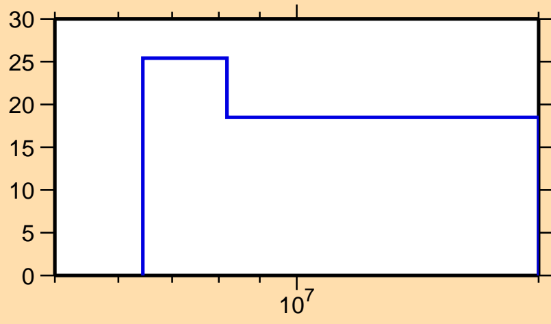
\Delta\sigma/\sigma vs. E for ^{71}\text{Ge}(n,2n)
