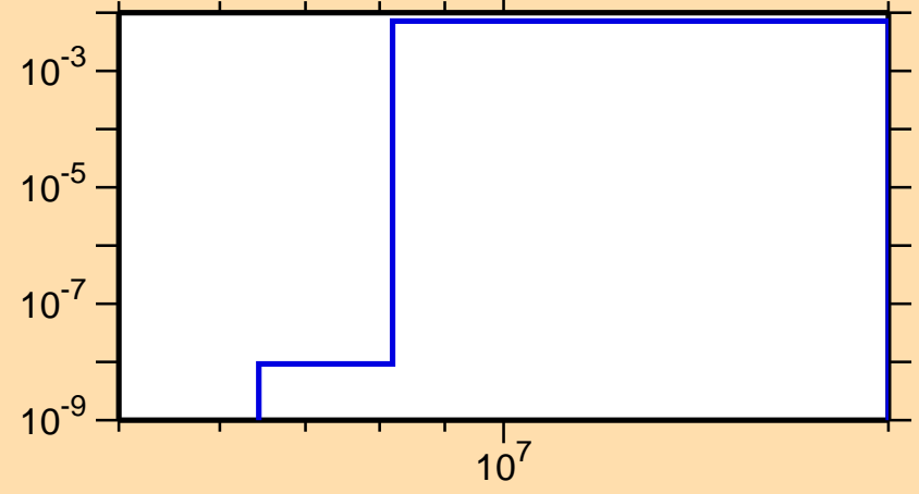
\sigma vs. E for ^{71}\text{Ge}(n,n\alpha)
