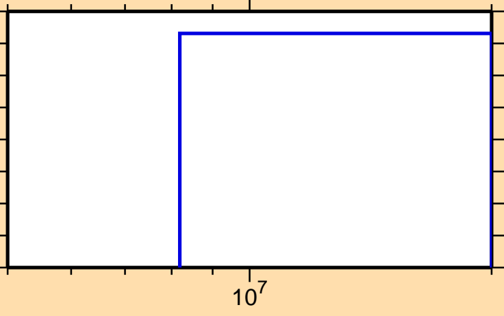
\sigma vs. E for ^{71}\text{Ge}(n,\text{He3})
