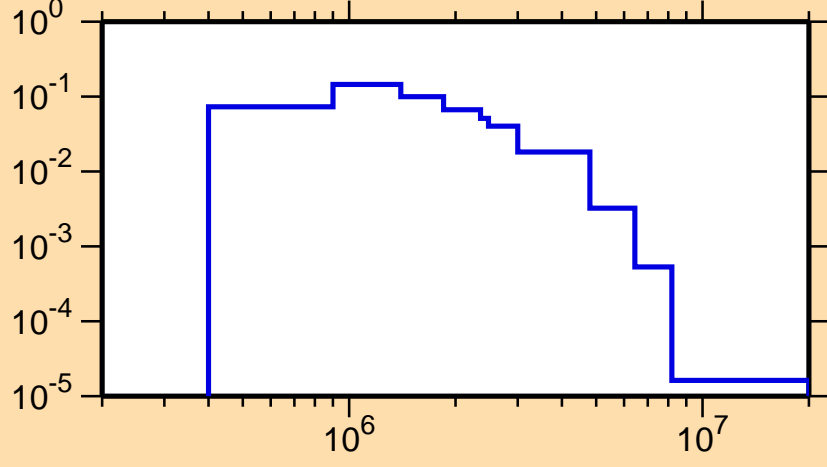
\sigma vs. E for ^{71}\text{Ge}(n,n_4)
