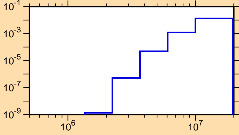
\sigma vs. E for ^{72}\text{Ge}(n,\alpha)
