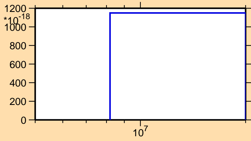
\sigma vs. E for ^{72}\text{Ge}(n,nt)
