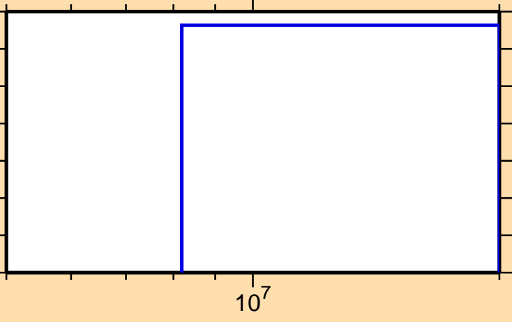
\sigma vs. E for ^{72}\text{Ge}(n,\text{He3})
