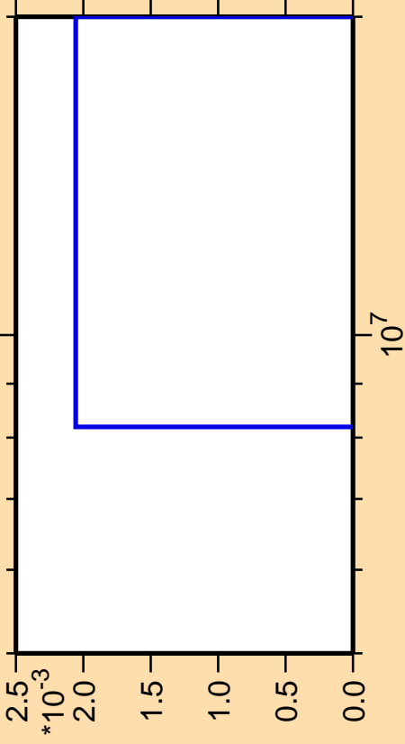
\Delta\sigma/\sigma vs. E for ^{72}\text{Ge}(n,2np)
