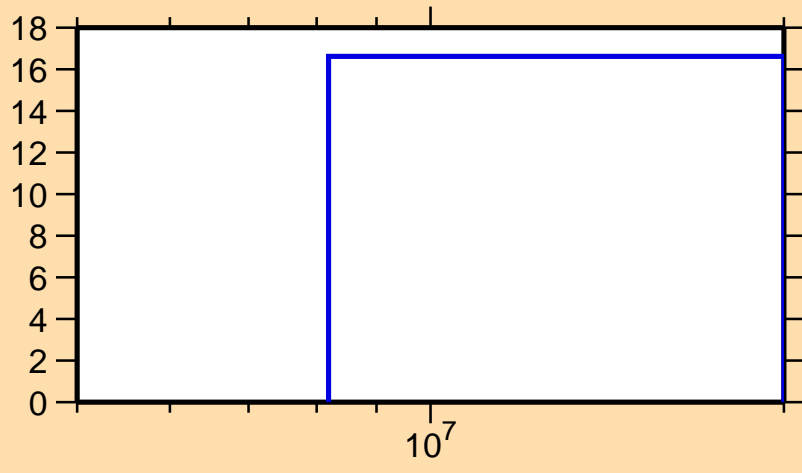
\Delta\sigma/\sigma vs. E for ^{72}\text{Ge}(n,2n)
