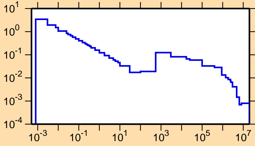
\sigma vs. E for ^{72}\text{Ge}(n,\gamma)
