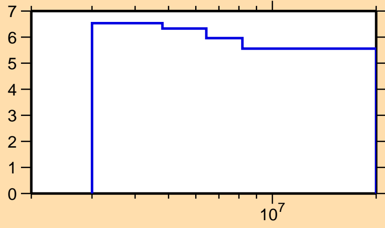
\Delta\sigma/\sigma vs. E for ^{72}\text{Ge}(n,n\text{nonel.})
