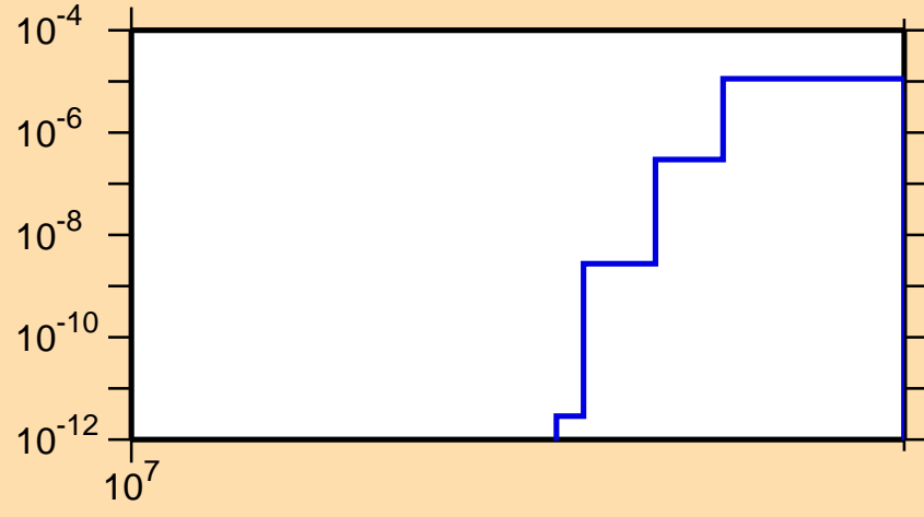
\sigma vs. E for ^{73}\text{Ge}(n,2n\alpha)
