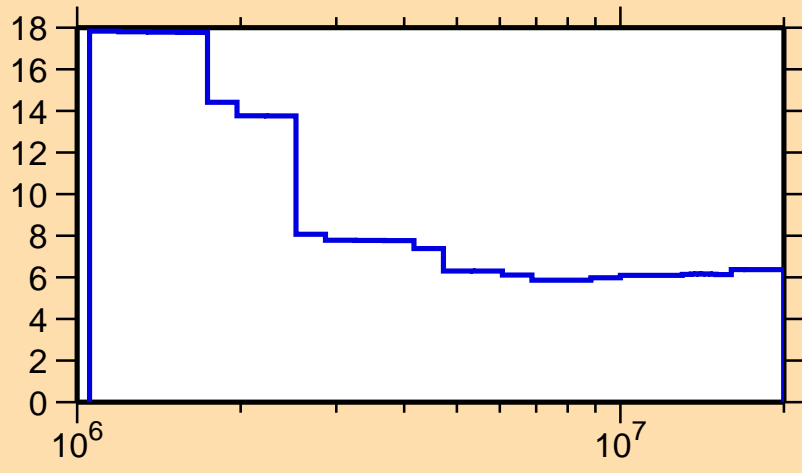
\Delta\sigma/\sigma vs. E for ^{73}\text{Ge}(n,n\text{onel.})
