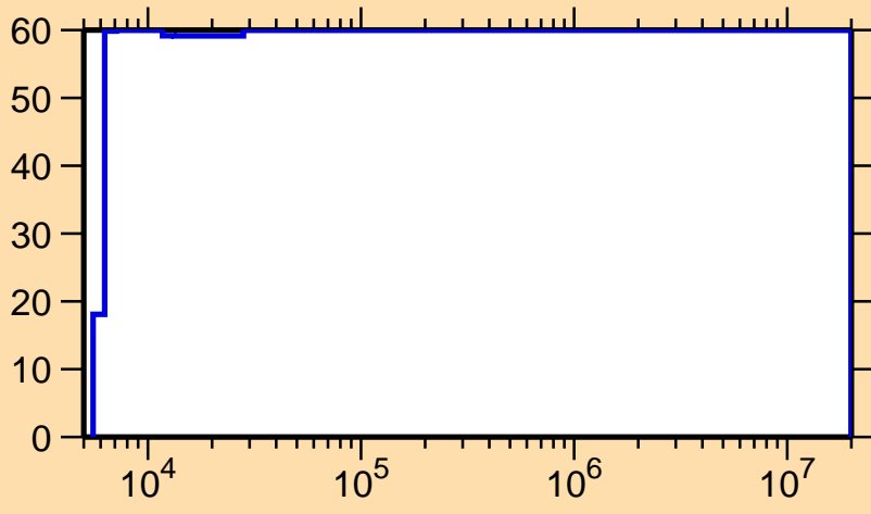
\Delta\sigma/\sigma vs. E for ^{73}\text{Ge}(n,\gamma)
