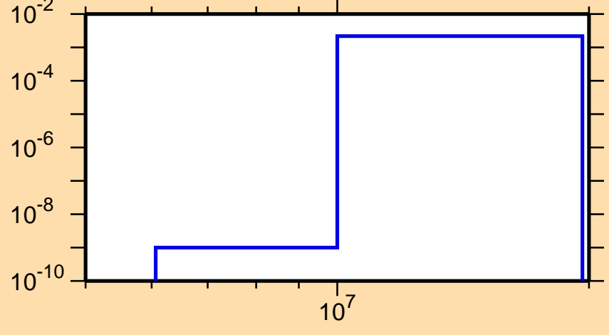
\sigma vs. E for ^{73}\text{Ge}(n,n\alpha)
