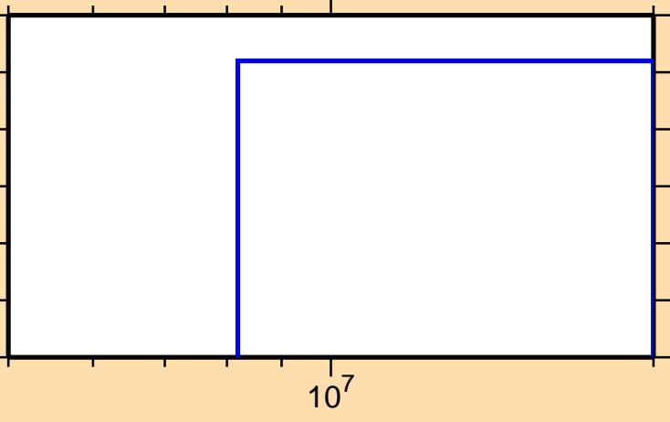
\sigma vs. E for ^{73}\text{Ge}(n,\text{pt})
