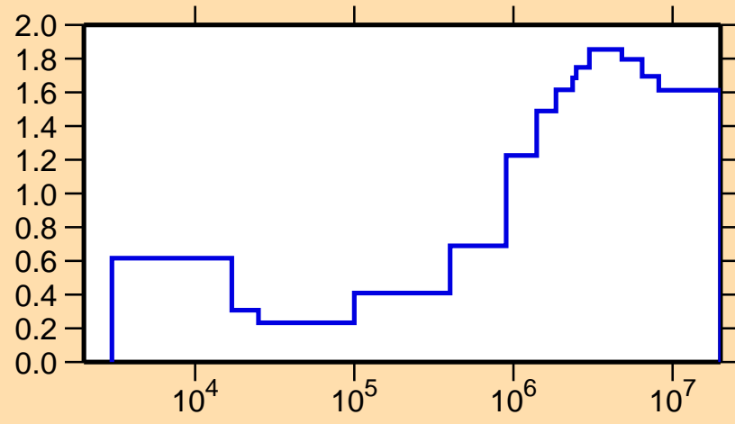
\sigma vs. E for ^{73}\text{Ge}(n,\text{nonel.})
