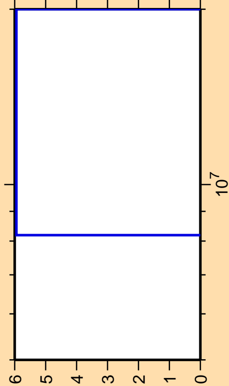
\Delta\sigma/\sigma vs. E for ^{73}\text{Ge}(n,nt)
