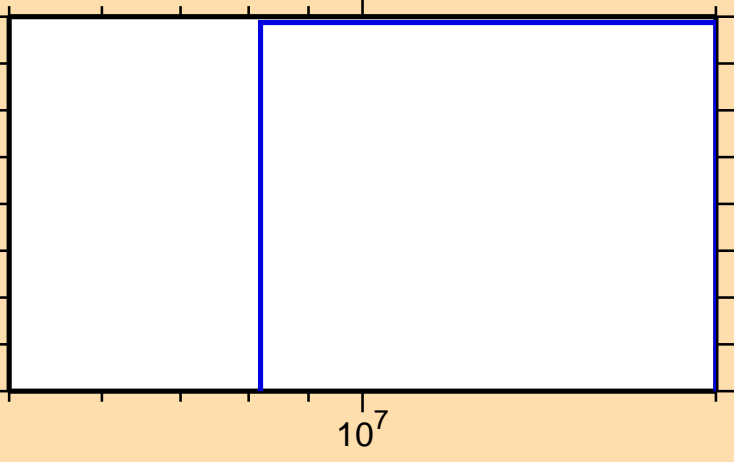
\sigma vs. E for ^{73}\text{Ge}(n,3n)
