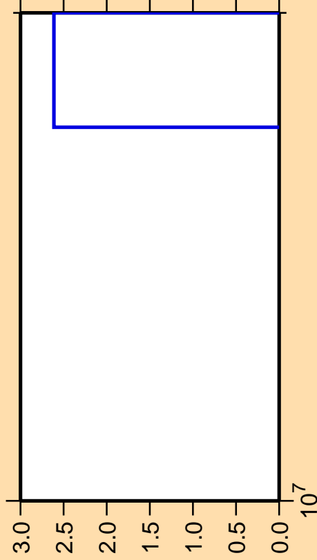
\Delta\sigma/\sigma vs. E for ^{74}\text{Ge}(n,nt)
