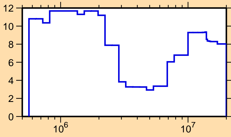
\Delta\sigma/\sigma vs. E for ^{74}\text{Ge}(n,\text{tot.})
