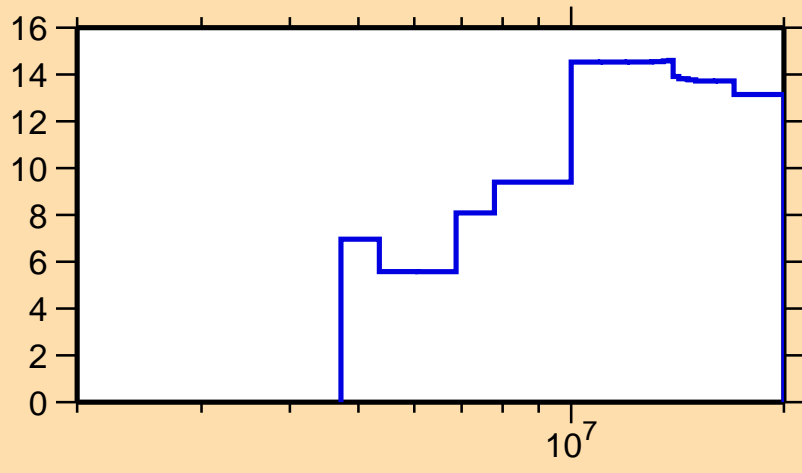
\Delta\sigma/\sigma vs. E for ^{74}\text{Ge}(n,el.)
