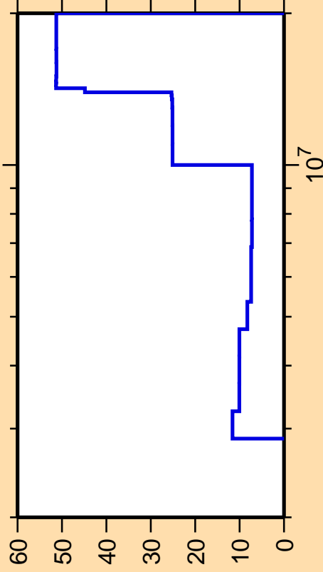
\Delta\sigma/\sigma vs. E for ^{74}\text{Ge}(n,n\text{cont.})
