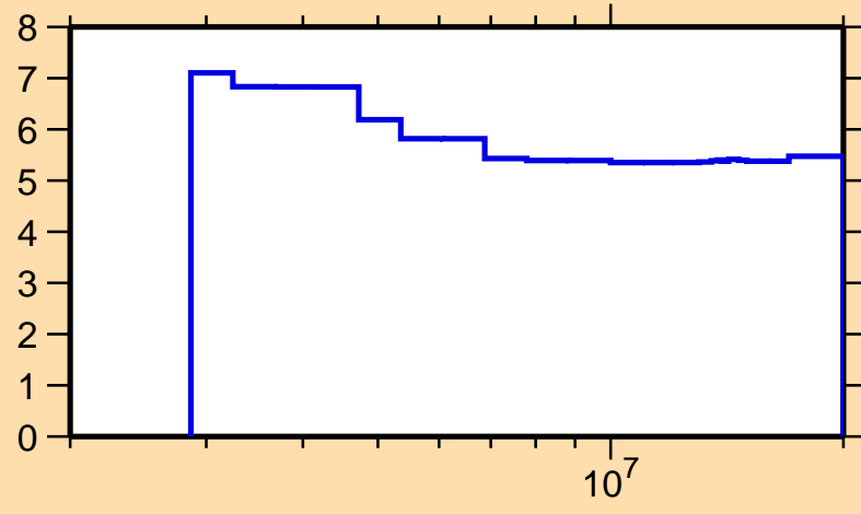
\Delta\sigma/\sigma vs. E for ^{74}\text{Ge}(n,n\text{inel.})
