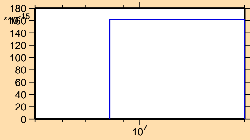
\sigma vs. E for ^{74}\text{Ge}(n,2n\alpha)
