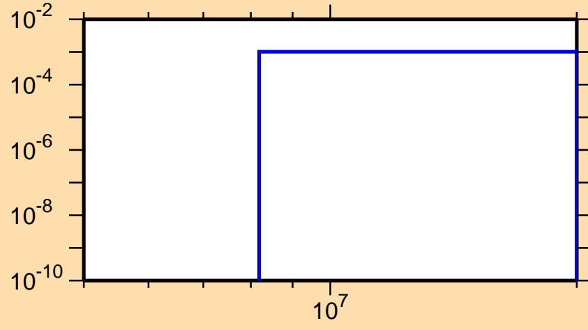
\sigma vs. E for ^{74}\text{Ge}(n,n\alpha)
