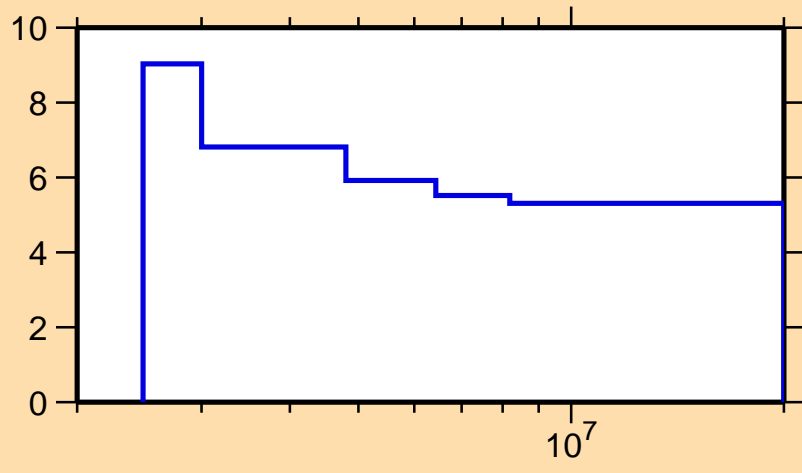
\Delta\sigma/\sigma vs. E for ^{74}\text{Ge}(n,n\text{onel.})
