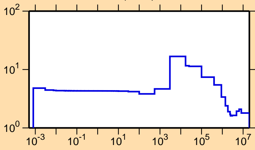
\sigma vs. E for ^{74}\text{Ge}(n,\text{el.})
