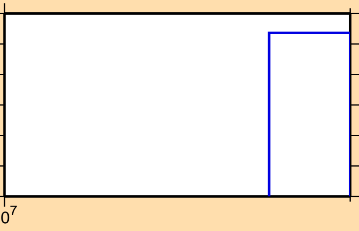
\sigma vs. E for ^{75}\text{Ge}(n,2np)
