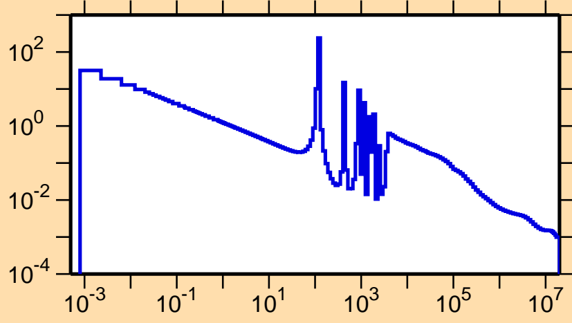
\sigma vs. E for ^{75}\text{Ge}(n,\gamma)
