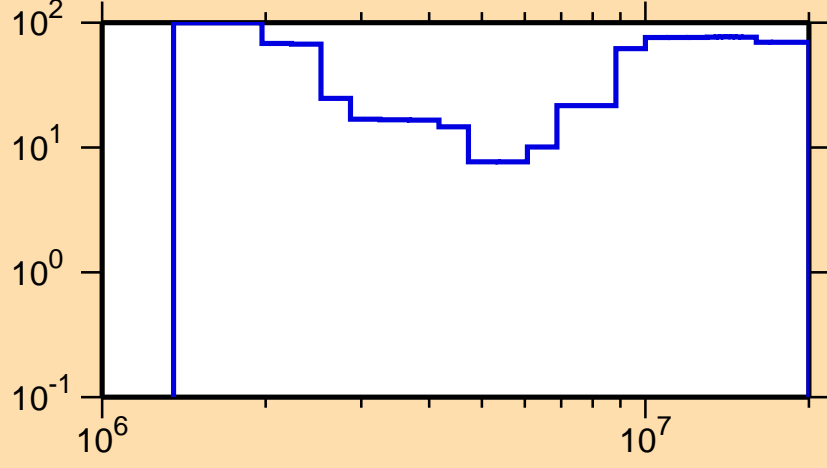
\Delta\sigma/\sigma vs. E for ^{75}\text{Ge}(n,n\text{cont.})
