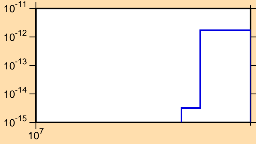
\sigma vs. E for ^{75}\text{Ge}(n,p\alpha)
