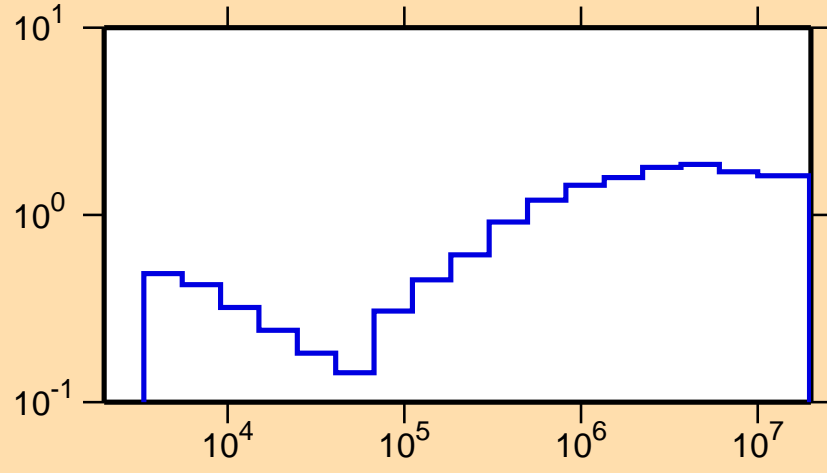
\sigma vs. E for ^{75}\text{Ge}(n,\text{nonel.})
