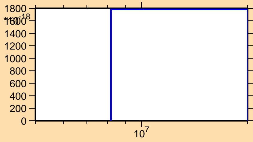
\sigma vs. E for ^{75}\text{Ge}(n,nt)
