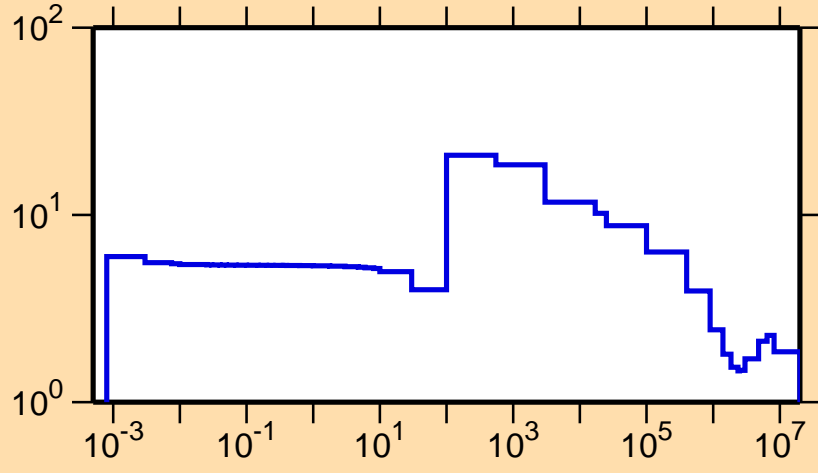
\sigma vs. E for ^{75}\text{Ge}(n,\text{el.})
