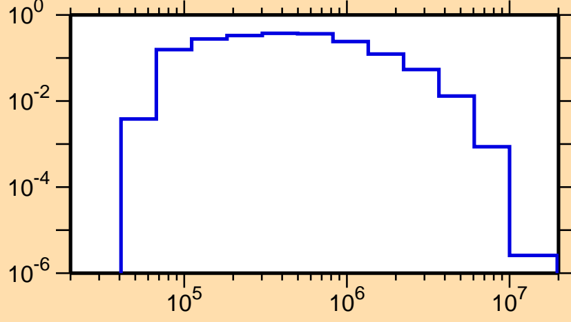
\sigma vs. E for ^{75}\text{Ge}(n,n_4)
