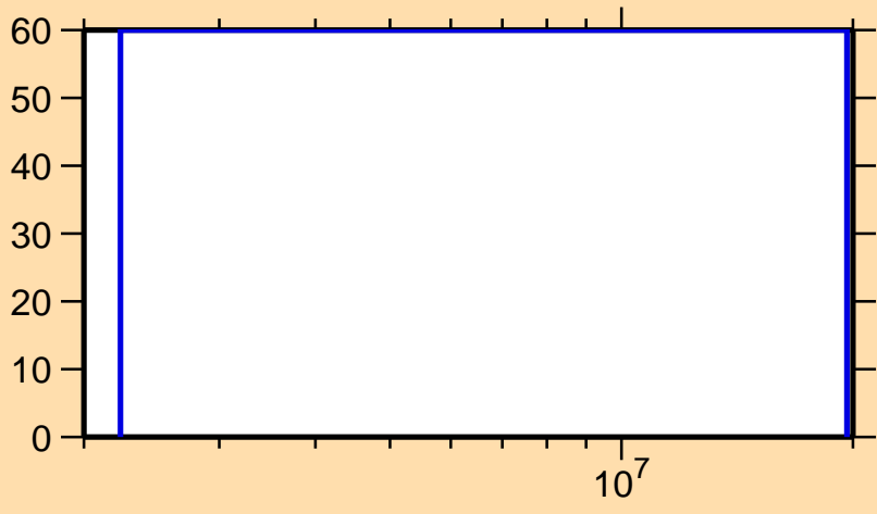
\Delta\sigma/\sigma vs. E for ^{75}\text{Ge}(n,p)
