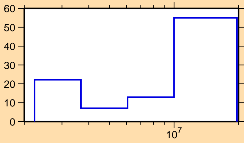
\Delta\sigma/\sigma vs. E for ^{75}\text{Ge}(n,ncont.)
