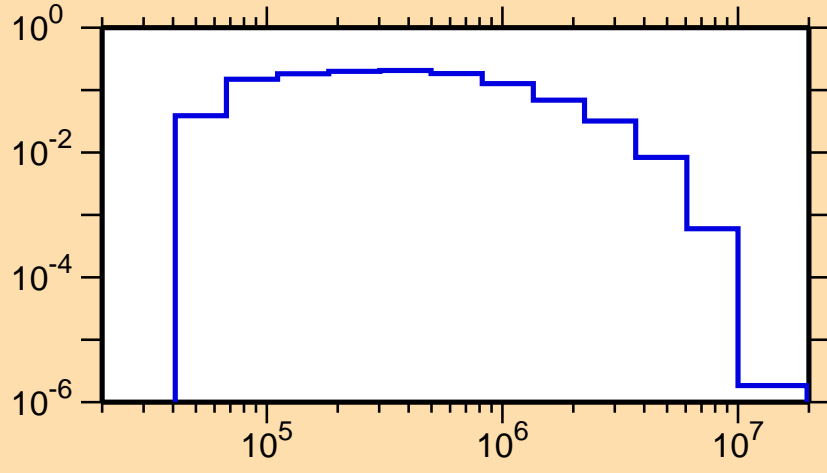
\sigma vs. E for ^{75}\text{Ge}(n,n_3)
