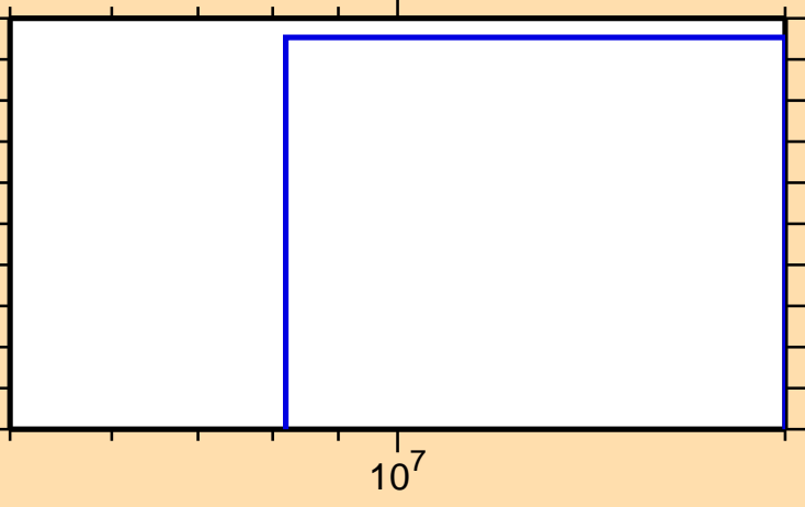
\sigma vs. E for ^{75}\text{Ge}(n,t)
