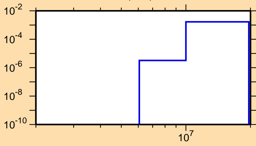
\sigma vs. E for ^{76}\text{Ge}(n,\alpha)
