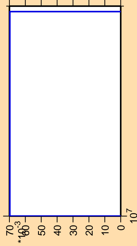
\Delta\sigma/\sigma vs. E for ^{76}\text{Ge}(n,nd)
