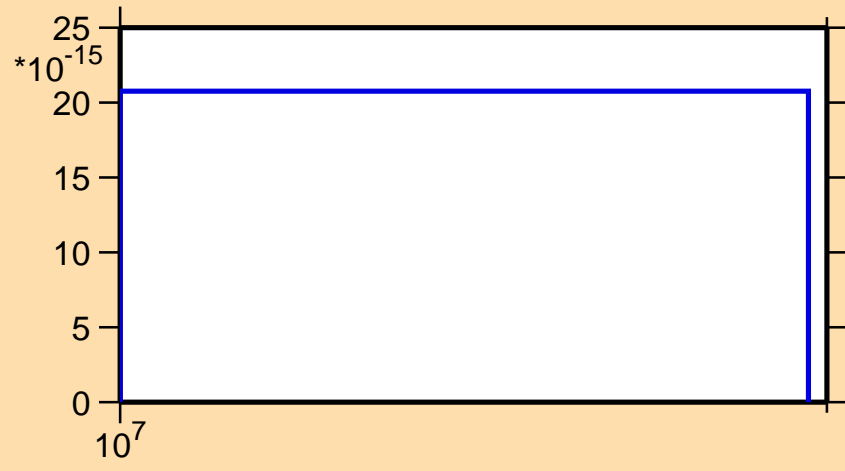
\sigma vs. E for ^{76}\text{Ge}(n,nd)
