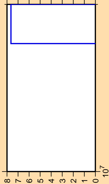
\Delta\sigma/\sigma vs. E for ^{77}\text{Ge}(n,nt)
