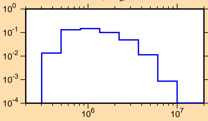
\sigma vs. E for ^{77}\text{Ge}(n,n_3)
