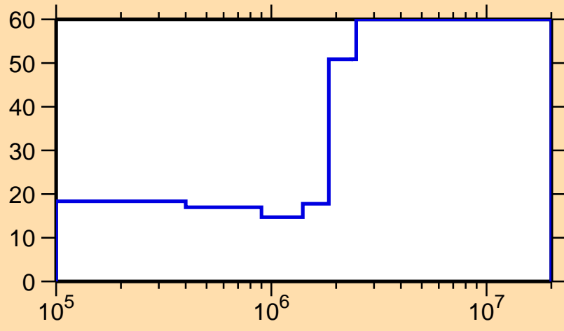
\Delta\sigma/\sigma vs. E for ^{77}\text{Ge}(n,n_1)
