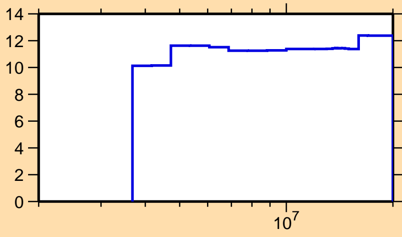
\Delta\sigma/\sigma vs. E for ^{78}\text{Ge}(n,n\text{nonel.})
