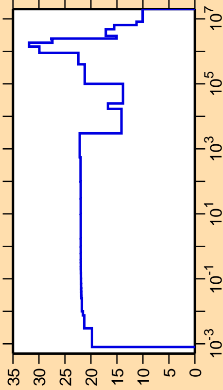
\Delta\sigma/\sigma vs. E for ^{78}\text{Ge}(n,\text{el.})
