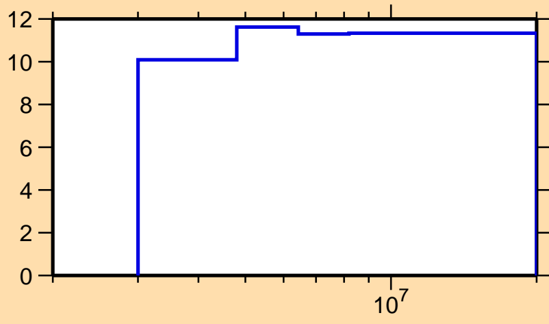
\Delta\sigma/\sigma vs. E for ^{78}\text{Ge}(n,n\text{onel.})
