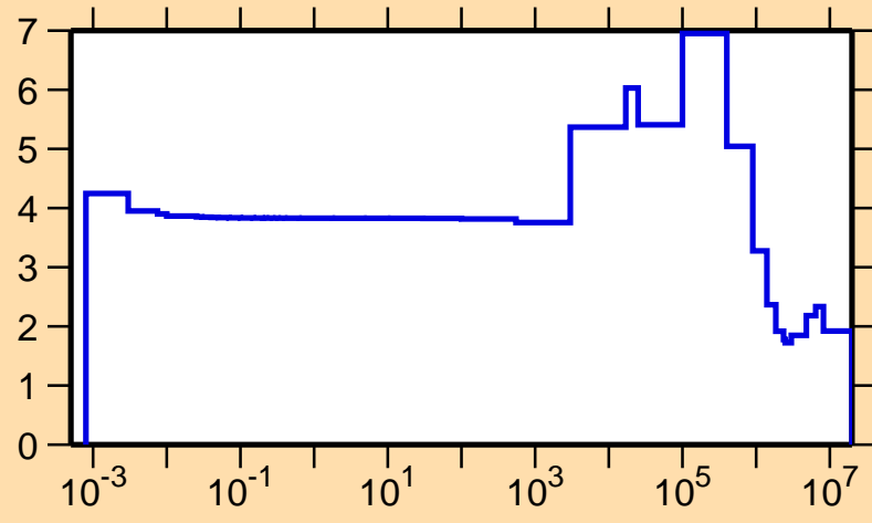
\sigma vs. E for ^{78}\text{Ge}(n,\text{el.})
