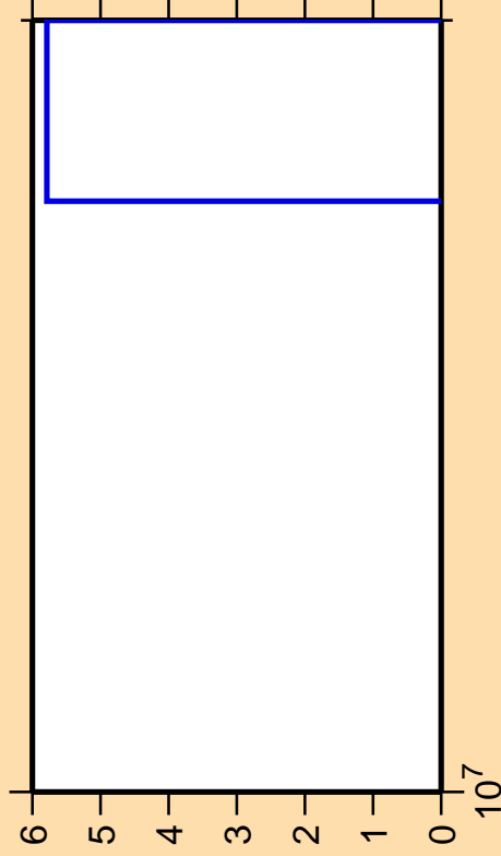
\Delta\sigma/\sigma vs. E for ^{79}\text{Ge}(n,nt)
