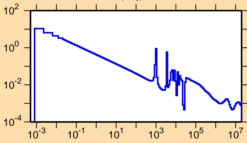
\sigma vs. E for ^{79}\text{Ge}(n,\gamma)
