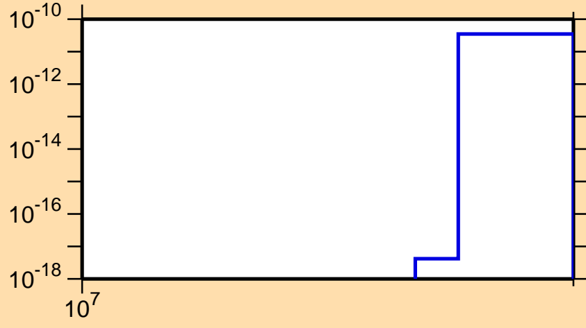
\sigma vs. E for ^{79}\text{Ge}(n,2n\alpha)
