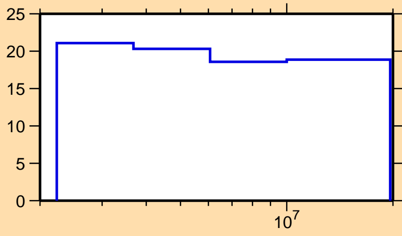
\Delta\sigma/\sigma vs. E for ^{79}\text{Ge}(n,n\text{inel.})
