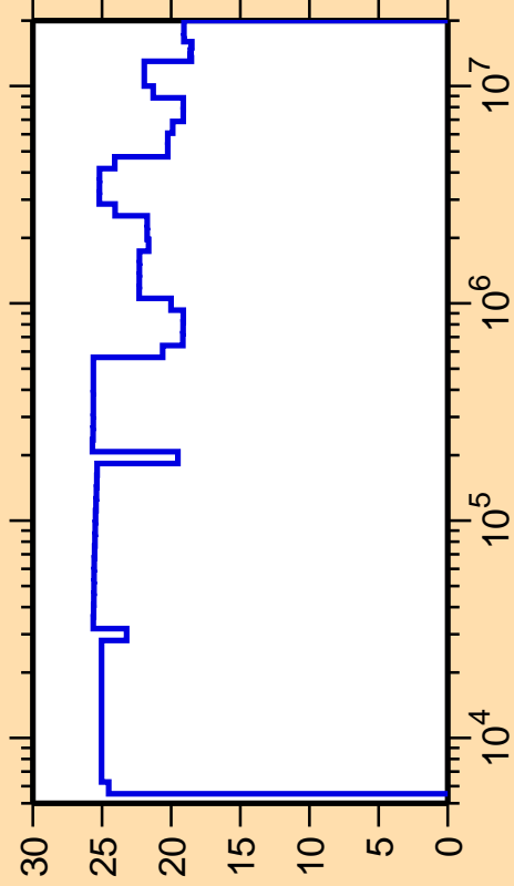
\Delta\sigma/\sigma vs. E for ^{79}\text{Ge}(n,\text{nonel.})
