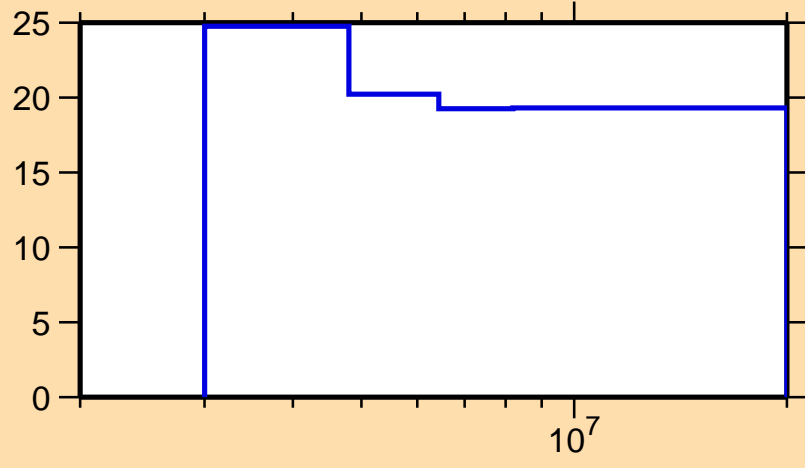
\Delta\sigma/\sigma vs. E for ^{79}\text{Ge}(n,n\text{inel.})
