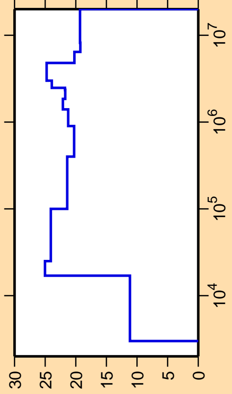
\Delta\sigma/\sigma vs. E for ^{79}\text{Ge}(n,\text{nonel.})
