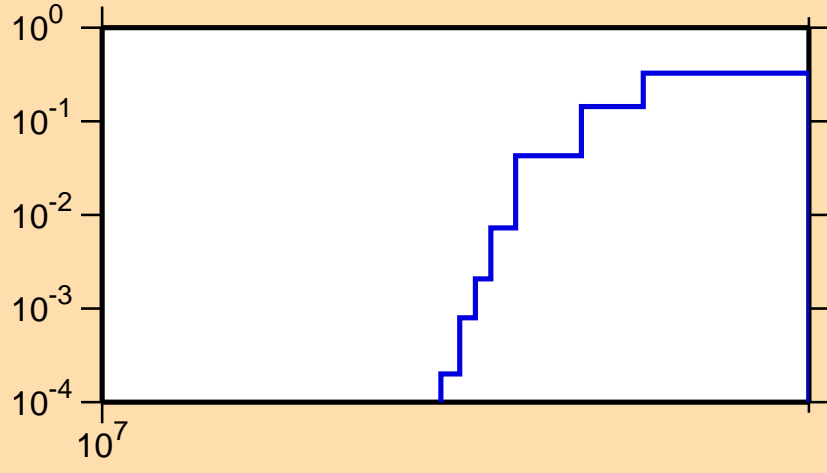
\sigma vs. E for ^{80}\text{Ge}(n,3n)
