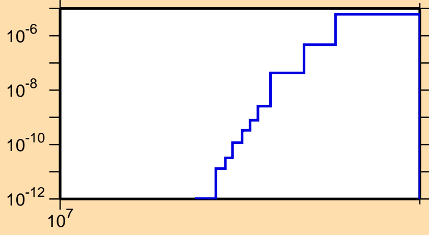
\sigma vs. E for ^{80}\text{Ge}(n,n\alpha)
