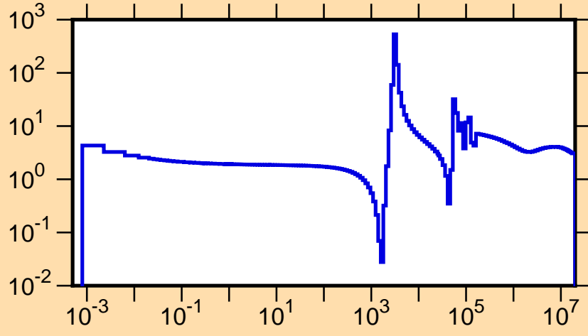
\sigma vs. E for ^{80}\text{Ge}(n,\text{tot.})
