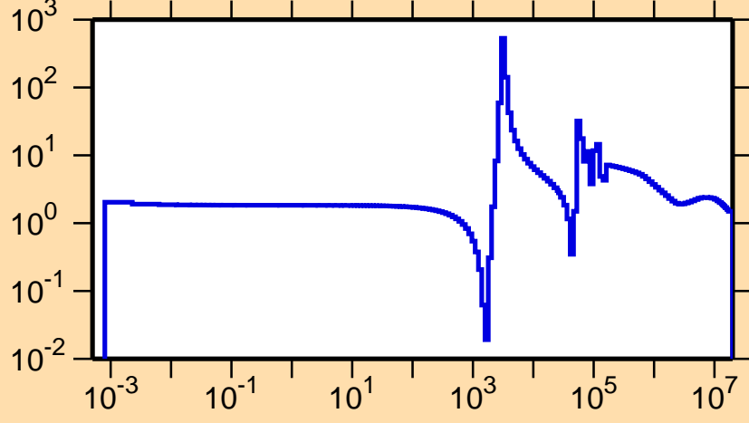
\sigma vs. E for ^{80}\text{Ge}(n,\text{el.})
