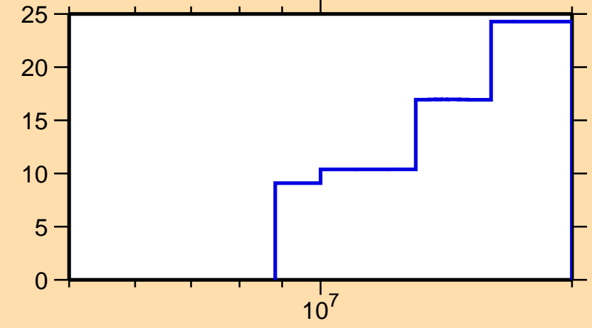
\Delta\sigma/\sigma vs. E for ^{80}\text{Ge}(n,\text{tot.})
