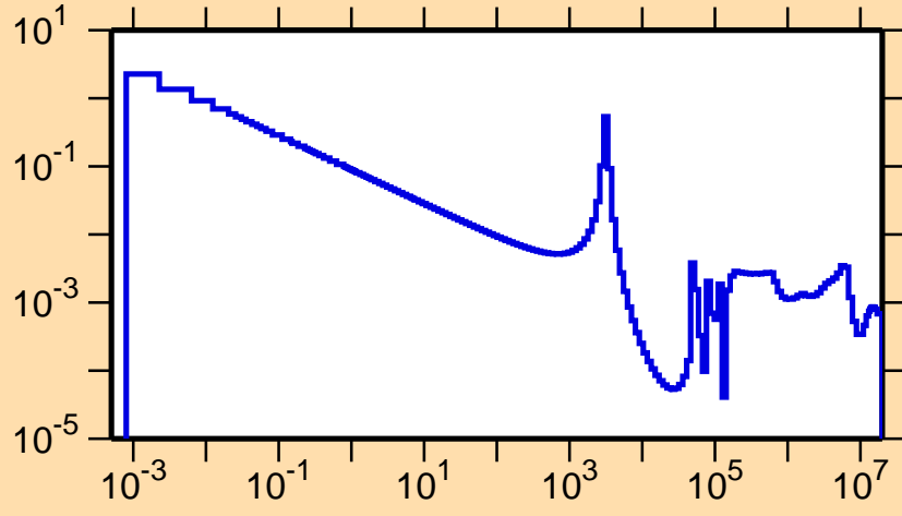
\sigma vs. E for ^{80}\text{Ge}(n,\gamma)
