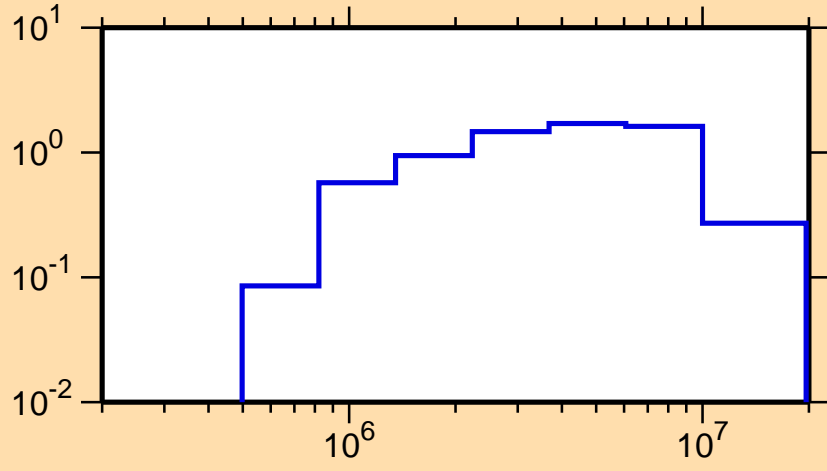
\sigma vs. E for ^{80}\text{Ge}(n,\text{inel.})
