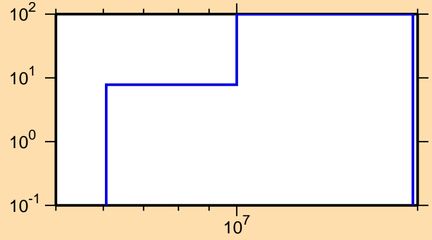
\Delta\sigma/\sigma vs. E for ^{80}\text{Ge}(n,ncont.)
