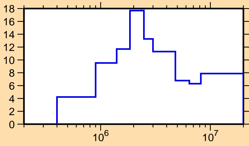
\Delta\sigma/\sigma vs. E for ^{80}\text{Ge}(n,\text{nonel.})
