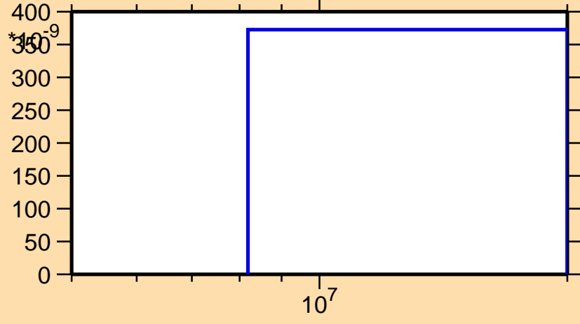
\sigma vs. E for ^{80}\text{Ge}(n,np)
