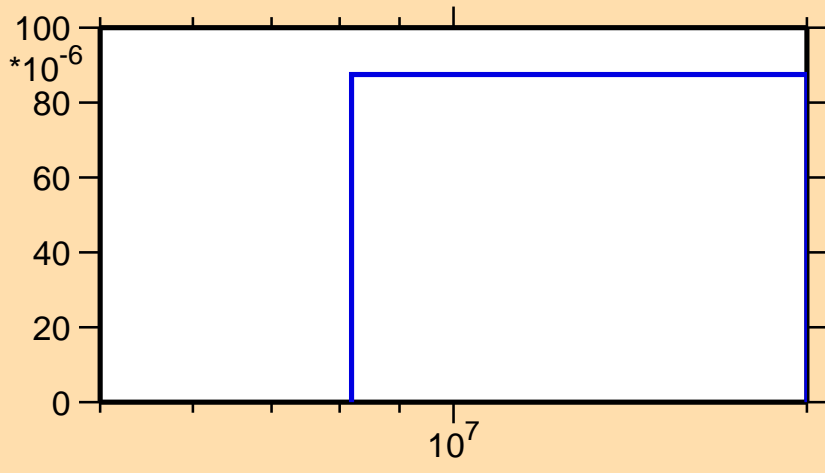
\sigma vs. E for ^{80}\text{Ge}(n,p)
