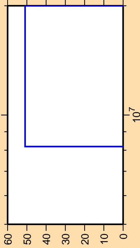
\Delta\sigma/\sigma vs. E for ^{80}\text{Ge}(n,3n)
