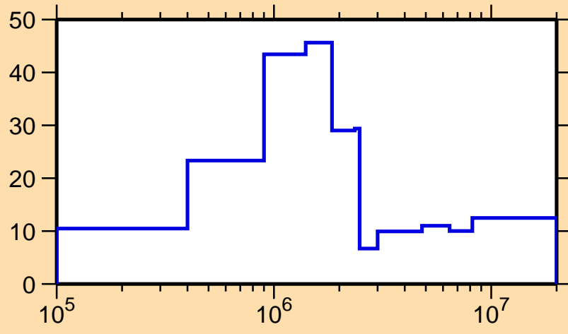
\Delta\sigma/\sigma vs. E for ^{80}\text{Ge}(n,\text{tot.})
