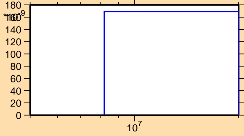
\sigma vs. E for ^{80}\text{Ge}(n,t)
