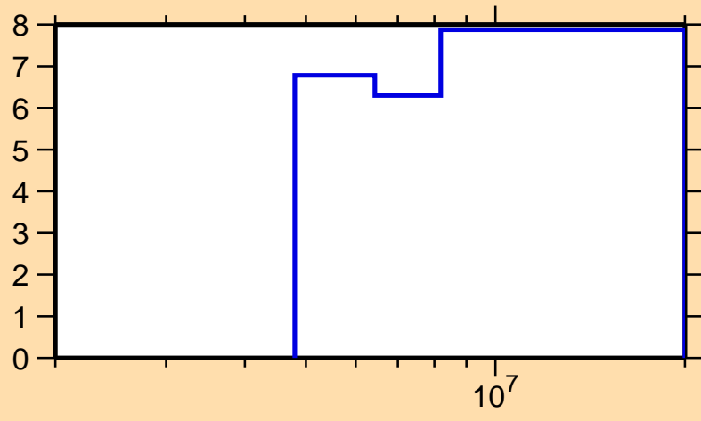
\Delta\sigma/\sigma vs. E for ^{80}\text{Ge}(n,n\text{onel.})
