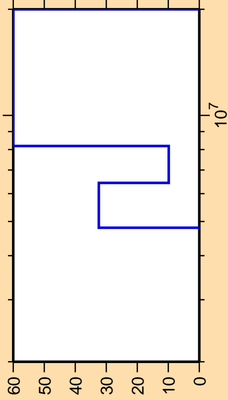
\Delta\sigma/\sigma vs. E for ^{80}\text{Ge}(n,n\text{cont.})
