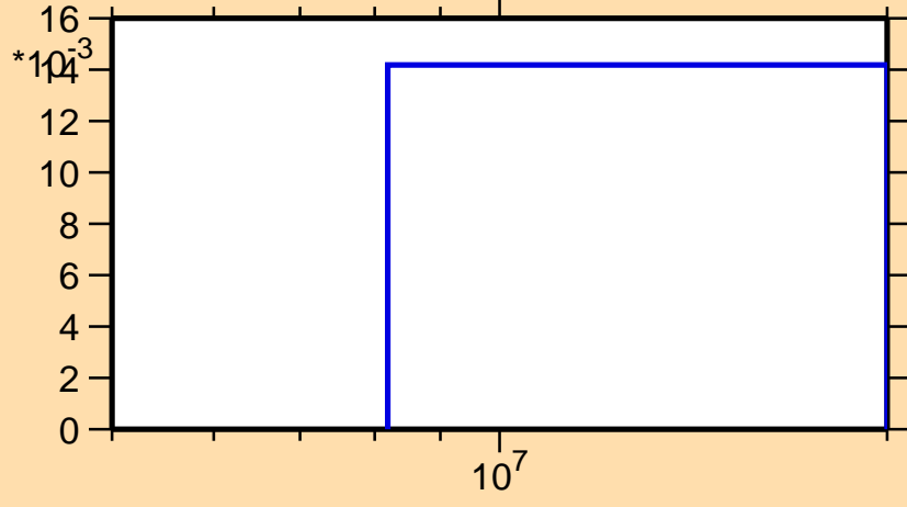
\sigma vs. E for ^{80}\text{Ge}(n,3n)
