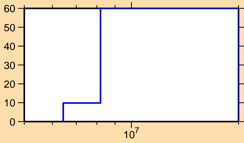
\Delta\sigma/\sigma vs. E for ^{80}\text{Ge}(n,n\text{cont.})
