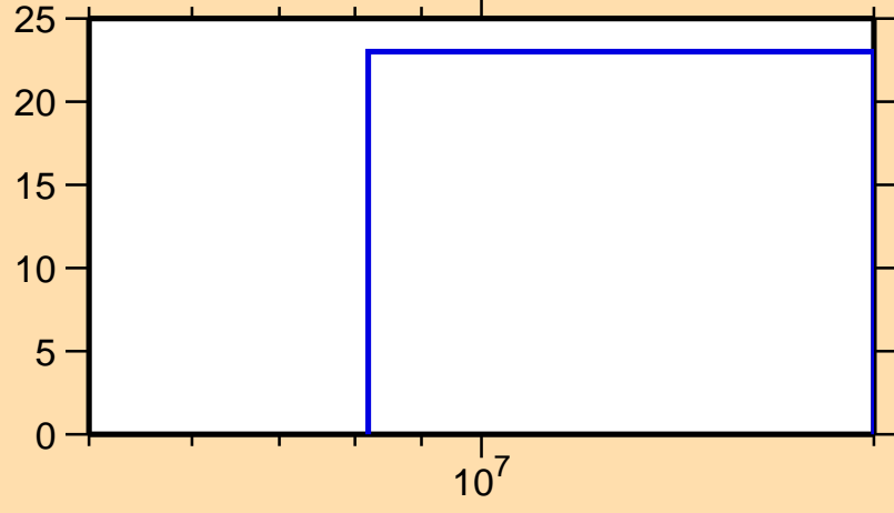
\Delta\sigma/\sigma vs. E for ^{80}\text{Ge}(n,el.)
