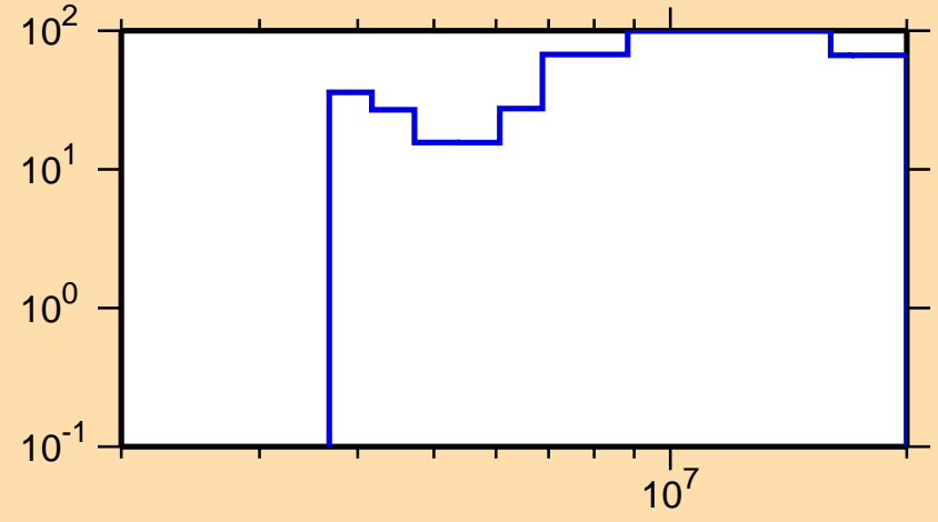
\Delta\sigma/\sigma vs. E for ^{81}\text{Ge}(n,n\text{cont.})
