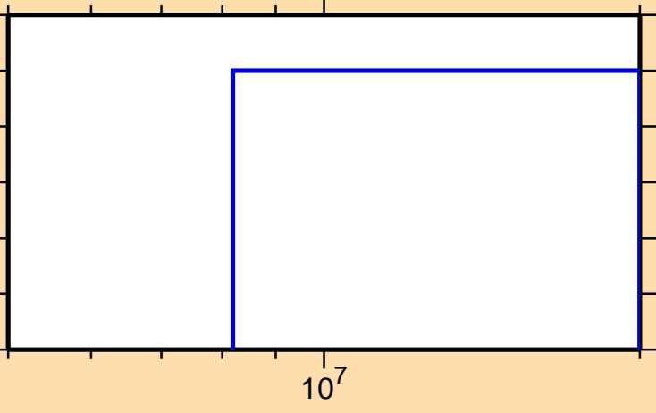
\sigma vs. E for ^{81}\text{Ge}(n,3n)
