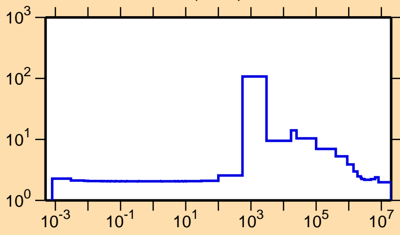
\sigma vs. E for ^{81}\text{Ge}(n,\text{el.})
