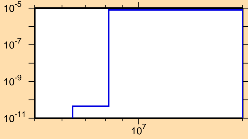
\sigma vs. E for ^{81}\text{Ge}(n,\alpha)
