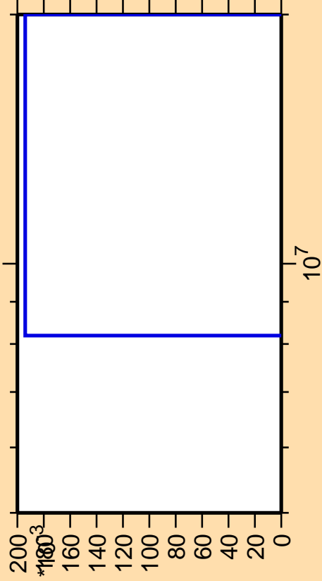
\Delta\sigma/\sigma vs. E for ^{81}\text{Ge}(n,2n\alpha)
