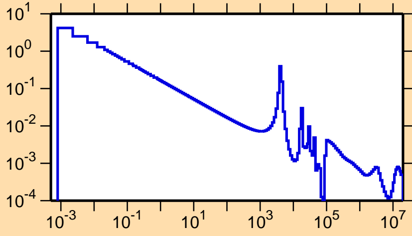
\sigma vs. E for ^{81}\text{Ge}(n,\gamma)
