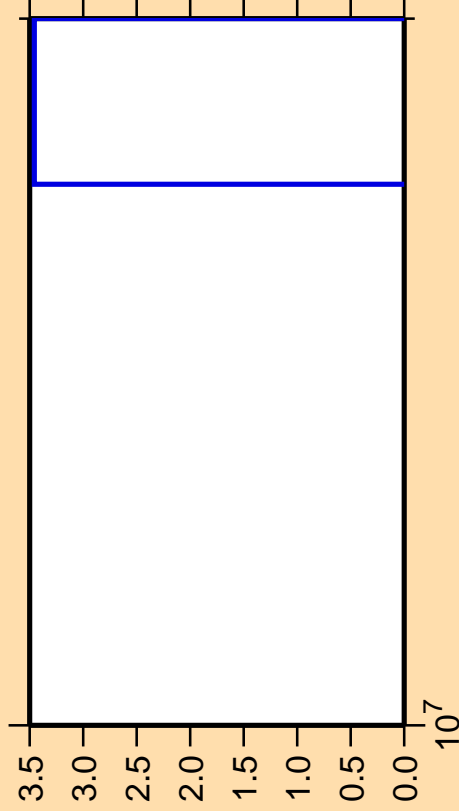
\Delta\sigma/\sigma vs. E for ^{81}\text{Ge}(n,2np)
