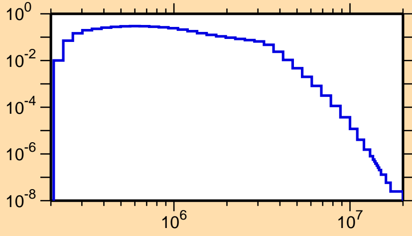
\sigma vs. E for ^{81}\text{Ge}(n,n_3)
