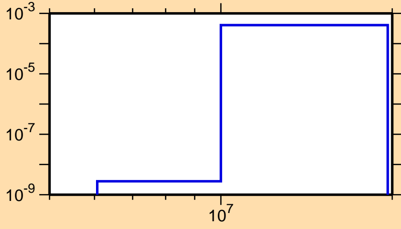
\sigma vs. E for ^{81}\text{Ge}(n,p)
