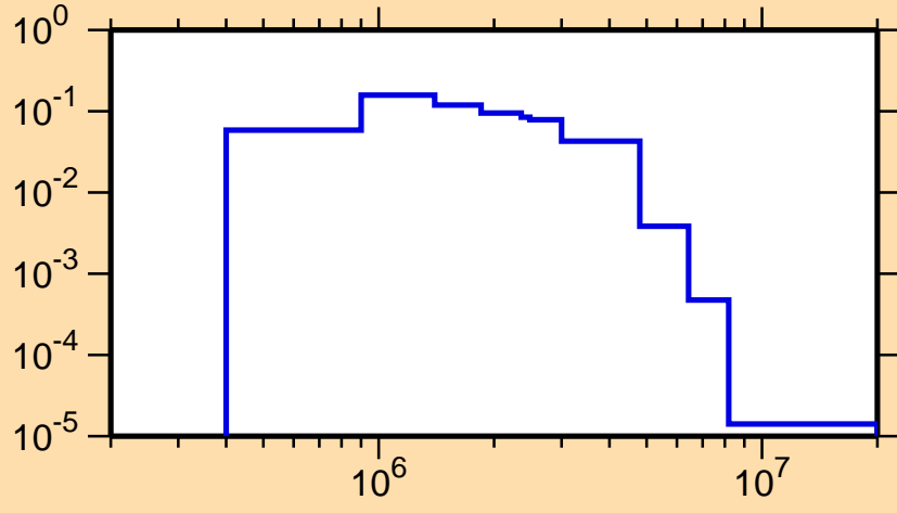
\sigma vs. E for ^{81}\text{Ge}(n,n_4)
