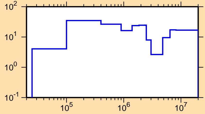
\Delta\sigma/\sigma vs. E for ^{81}\text{Ge}(n,\text{tot.})
