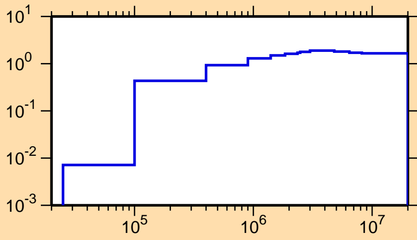
\sigma vs. E for ^{81}\text{Ge}(n,\text{nonel.})
