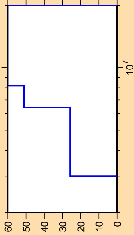
\Delta\sigma/\sigma vs. E for ^{82}\text{Ge}(n,n\text{cont.})
