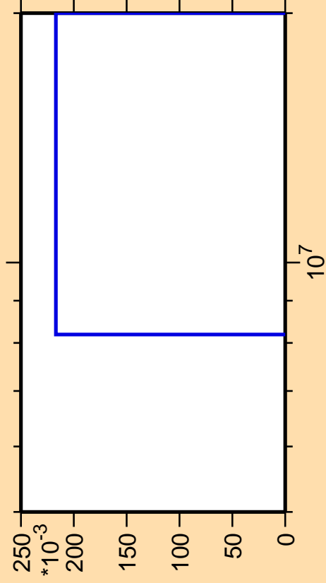
\Delta\sigma/\sigma vs. E for ^{82}\text{Ge}(n,nt)
