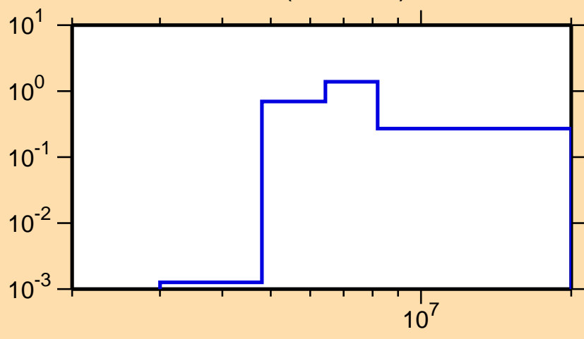
\sigma vs. E for ^{82}\text{Ge}(n,n\text{cont.})
