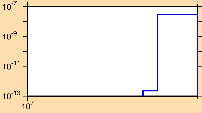
\sigma vs. E for ^{83}\text{Ge}(n,\text{nd})
