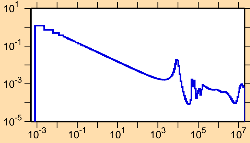
\sigma vs. E for ^{83}\text{Ge}(n,\gamma)
