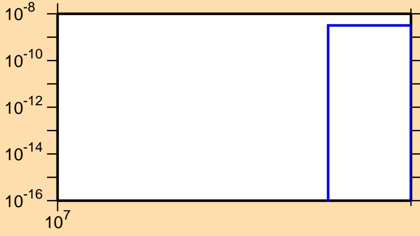
\sigma vs. E for ^{83}\text{Ge}(n,nt)
