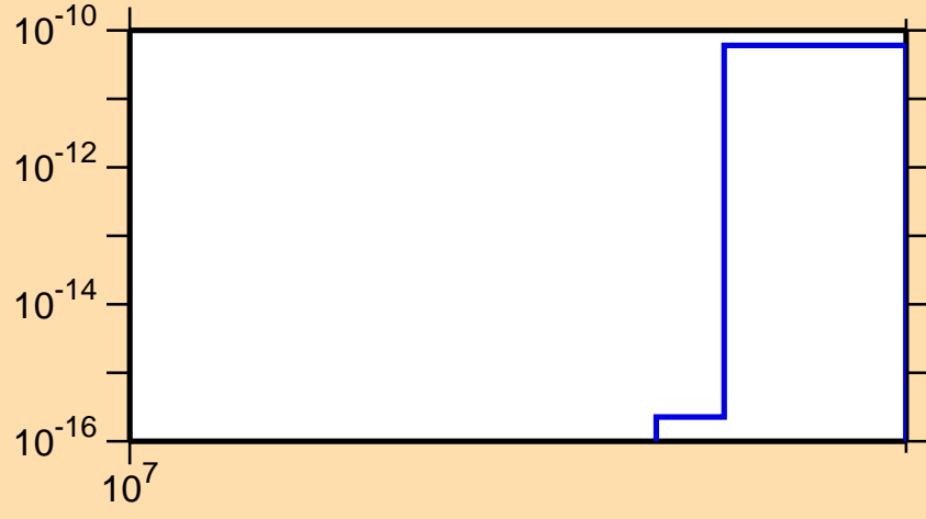
\sigma vs. E for ^{83}\text{Ge}(n,2n\alpha)
