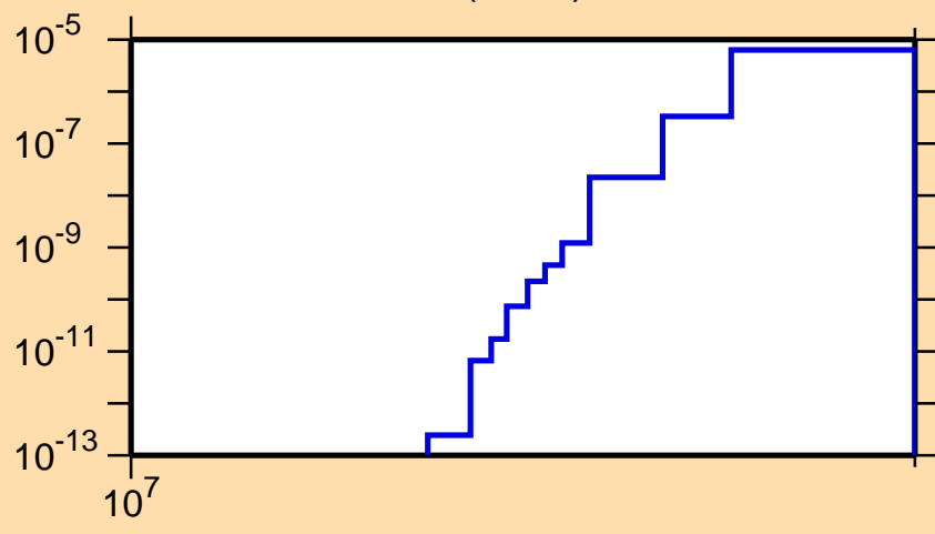
\sigma vs. E for ^{83}\text{Ge}(n,\alpha)
