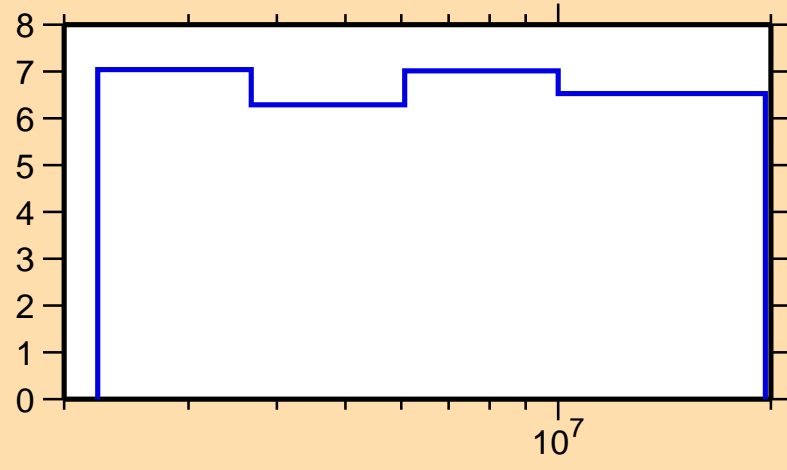
\Delta\sigma/\sigma vs. E for ^{83}\text{Ge}(n,n\text{onel.})
