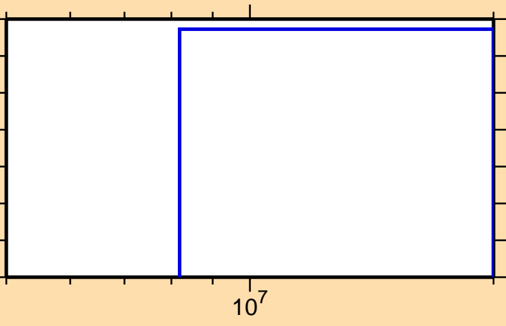
\sigma vs. E for ^{83}\text{Ge}(n,n\alpha)
