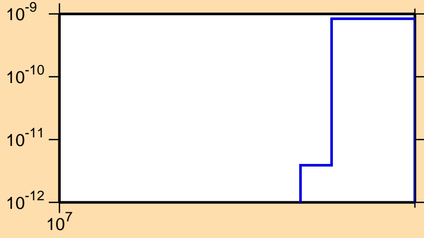
\sigma vs. E for ^{154}\text{Hf}(n,2n\alpha)
