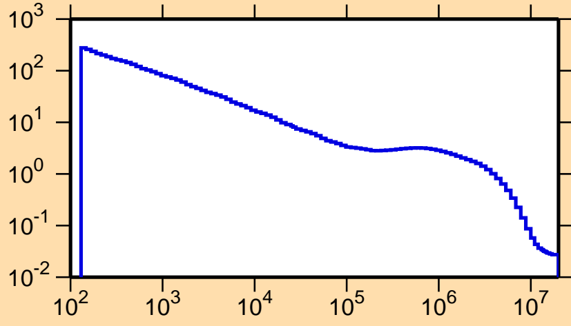
\sigma vs. E for ^{154}\text{Hf}(n,p)
