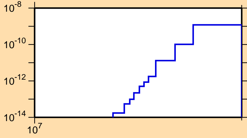
\sigma vs. E for ^{154}\text{Hf}(\text{mt } 34)
