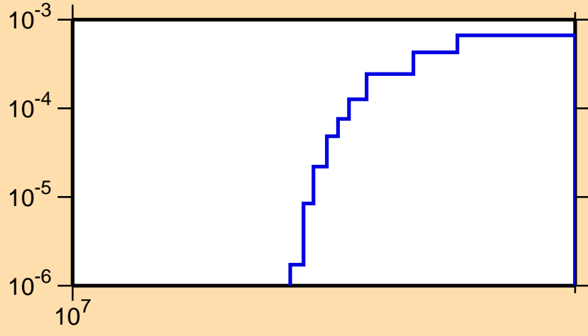
\sigma vs. E for ^{154}\text{Hf}(n,2n)
