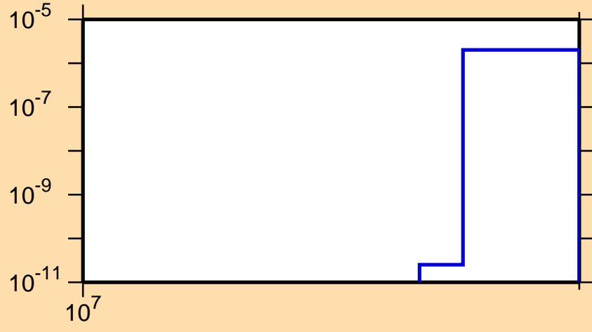
\sigma vs. E for ^{154}\text{Hf}(n,2np)
