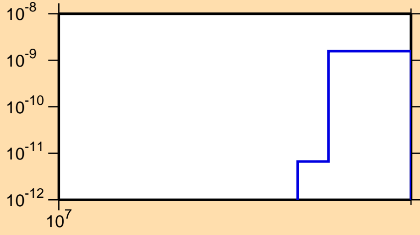
\sigma vs. E for ^{154}\text{Hf}(n,\text{nd})
