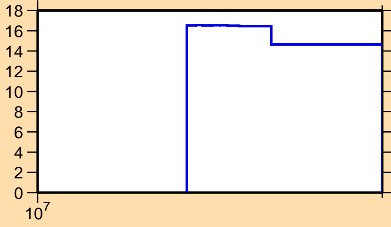
\Delta\sigma/\sigma vs. E for ^{154}\text{Hf}(n,\text{nonel.})
