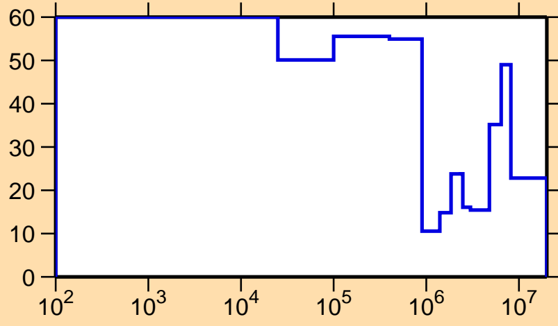
\Delta\sigma/\sigma vs. E for ^{154}\text{Hf}(n,\text{el.})
