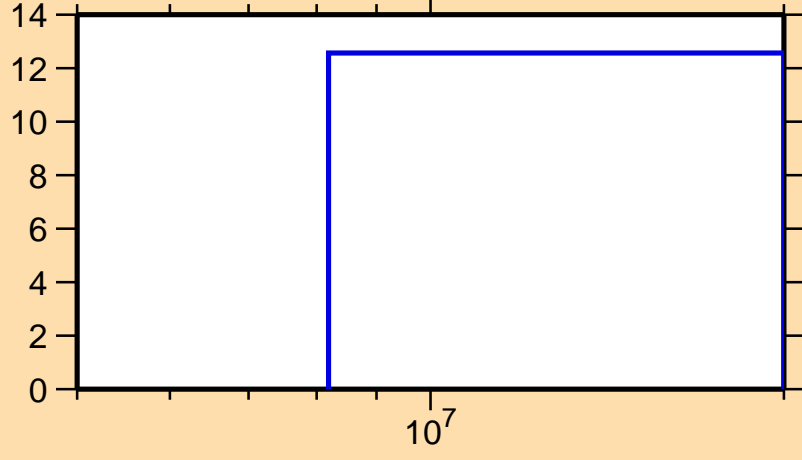
\Delta\sigma/\sigma vs. E for ^{154}\text{Hf}(n,\text{tot.})
