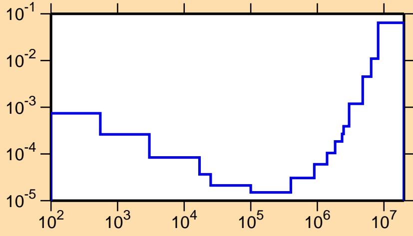
\sigma vs. E for ^{154}\text{Hf}(n,p\alpha)
