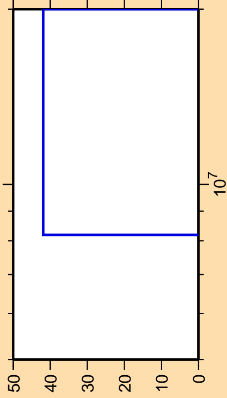
\Delta\sigma/\sigma vs. E for ^{154}\text{Hf}(n,2n\alpha)
