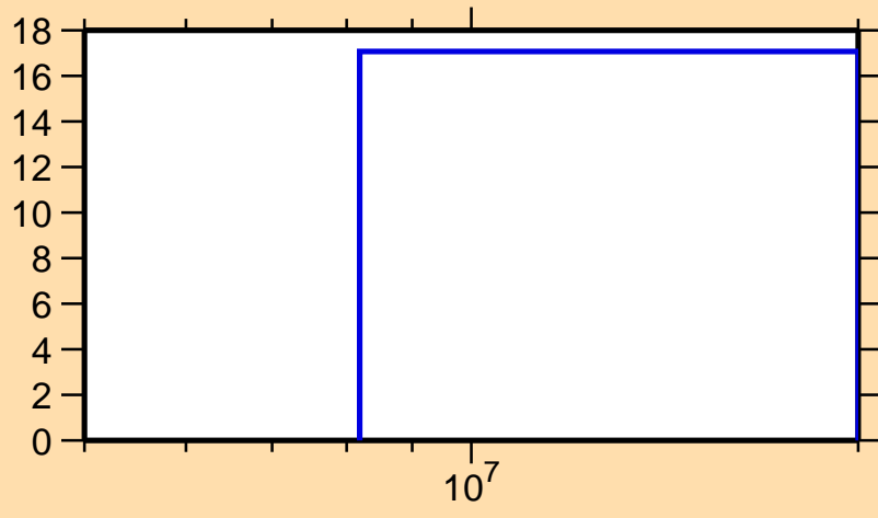
\Delta\sigma/\sigma vs. E for ^{154}\text{Hf}(n,\text{nonel.})
