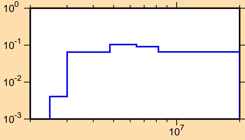
\sigma vs. E for ^{154}\text{Hf}(n,n\text{cont.})
