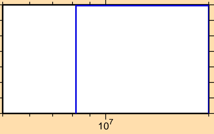
\sigma vs. E for ^{154}\text{Hf}(n,2n)
