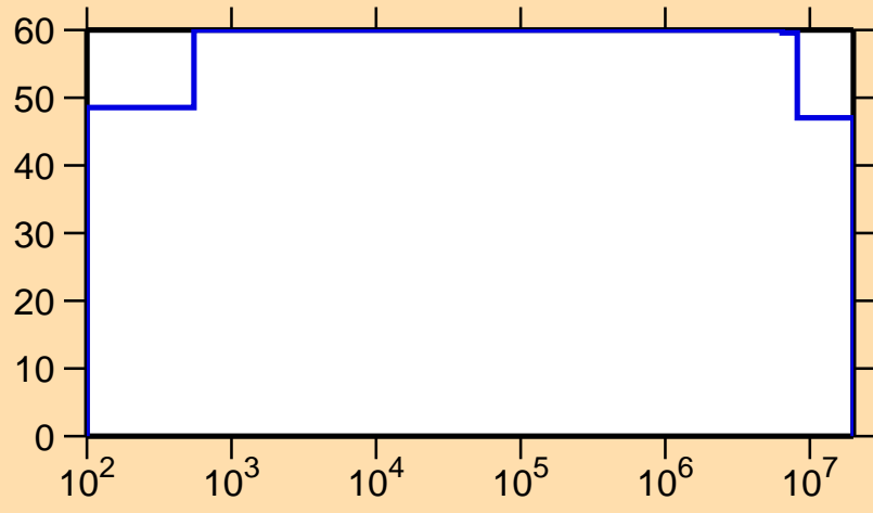
\Delta\sigma/\sigma vs. E for ^{154}\text{Hf}(n,\gamma)
