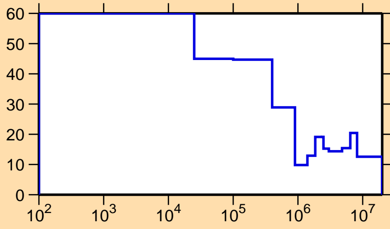
\Delta\sigma/\sigma vs. E for ^{154}\text{Hf}(n,\text{tot.})
