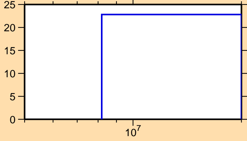
\Delta\sigma/\sigma vs. E for ^{154}\text{Hf}(n,\text{el.})
