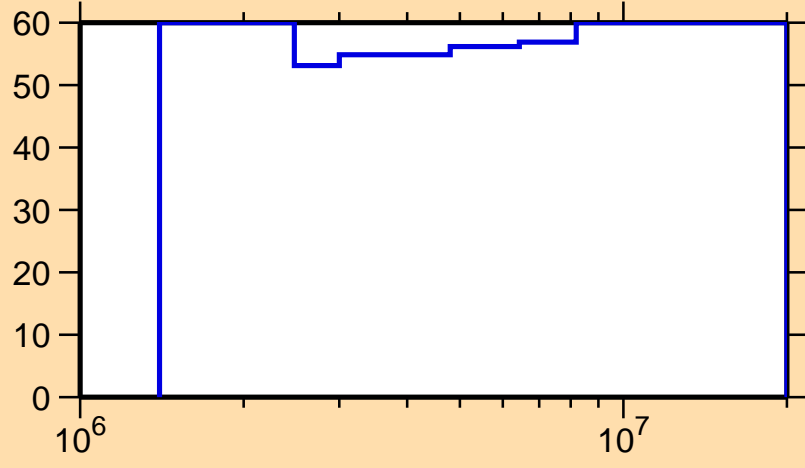
\Delta\sigma/\sigma vs. E for ^{154}\text{Hf}(n,\text{inel.})
