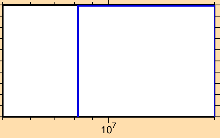
\sigma vs. E for ^{154}\text{Hf}(n,t)
