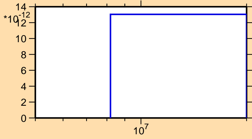
\sigma vs. E for ^{154}\text{Hf}(n,\text{nd})
