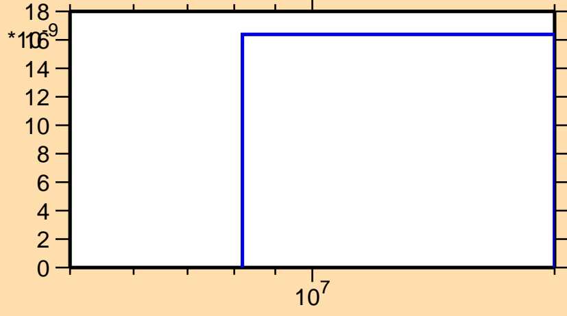
\sigma vs. E for ^{154}\text{Hf}(n,2np)
