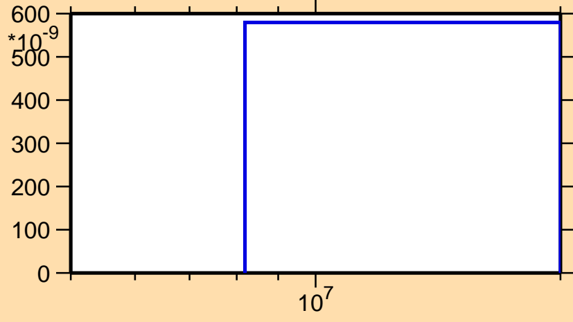
\sigma vs. E for ^{154}\text{Hf}(n,\text{pt})
