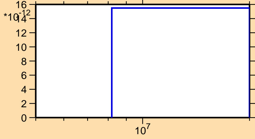
\sigma vs. E for ^{154}\text{Hf}(\text{mt } 34)
