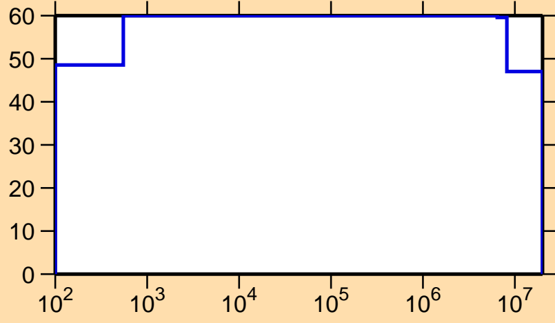
\Delta\sigma/\sigma vs. E for ^{154}\text{Hf}(n,\gamma)
