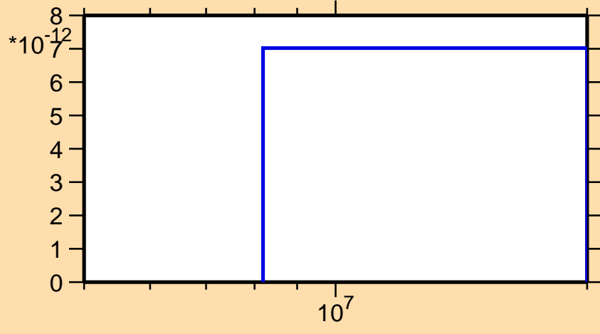
\sigma vs. E for ^{154}\text{Hf}(n,2n\alpha)
