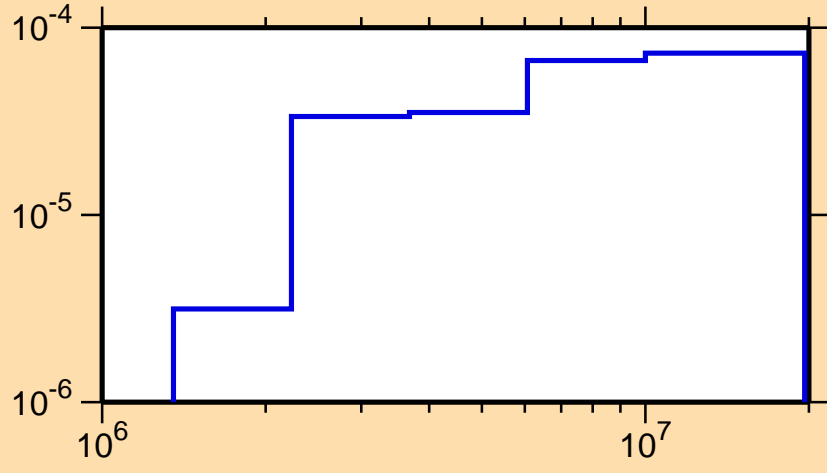
\sigma vs. E for ^{159}\text{Hf}(n,n_4)
