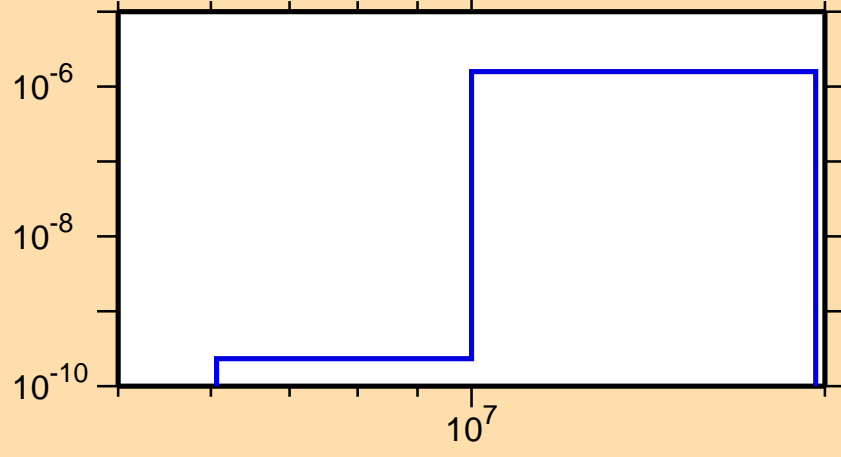
\sigma vs. E for ^{159}\text{Hf}(\text{mt117})
