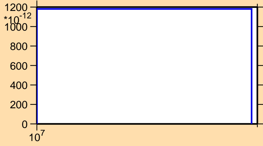
\sigma vs. E for ^{159}\text{Hf} (mt 34)
