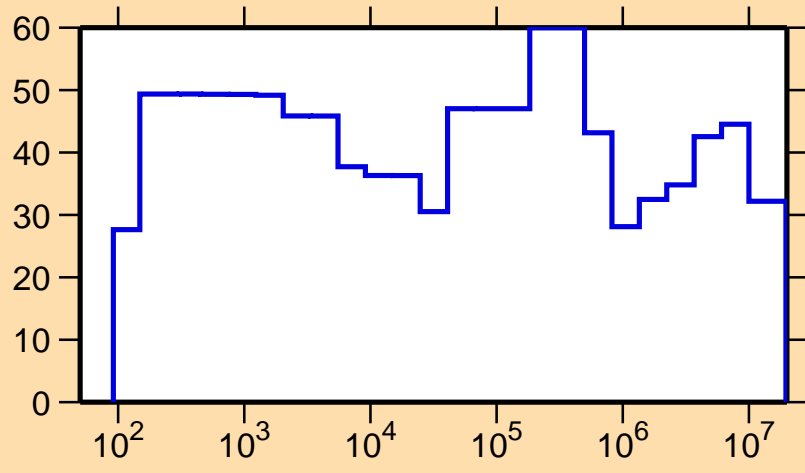
\Delta\sigma/\sigma vs. E for ^{159}\text{Hf}(n,\text{el.})
