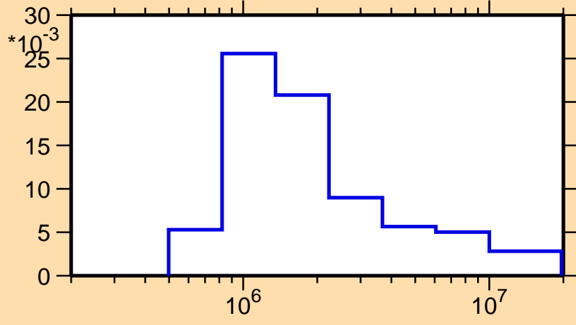
\sigma vs. E for ^{159}\text{Hf}(n,n_2)
