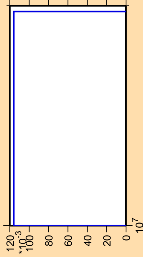
\Delta\sigma/\sigma vs. E for ^{159}\text{Hf}(n,nt)
