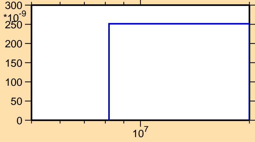
\sigma vs. E for ^{159}\text{Hf}(n,nd)
