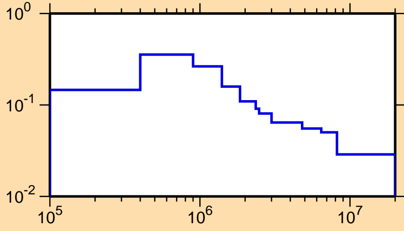
\sigma vs. E for ^{159}\text{Hf}(n,n_1)
