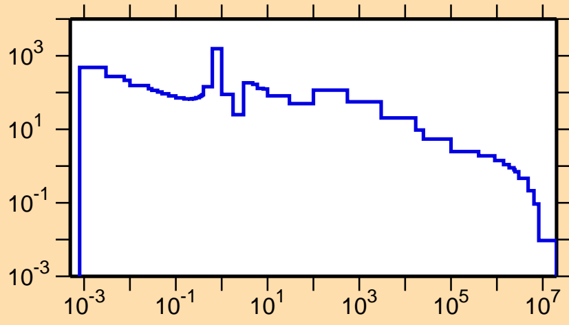
\sigma vs. E for ^{159}\text{Hf}(n,\gamma)
