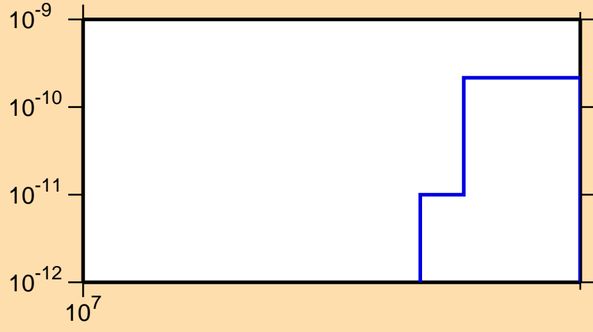
\sigma vs. E for ^{160}\text{Hf} (mt 34)
