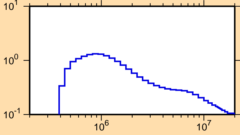
\sigma vs. E for ^{160}\text{Hf}(n,n_1)
