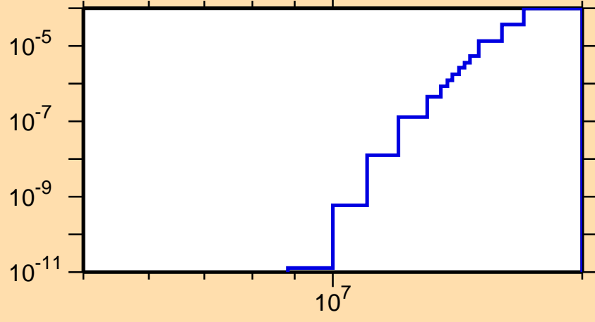
\sigma vs. E for ^{160}\text{Hf}(n,\text{pd})
