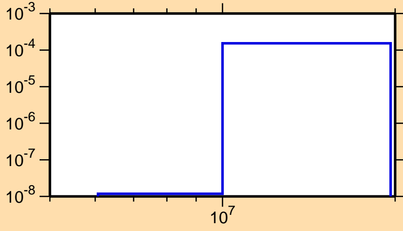
\sigma vs. E for ^{160}\text{Hf} (mt 45)
