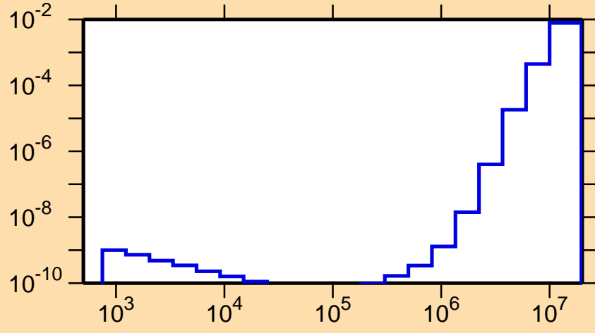
\sigma vs. E for ^{160}\text{Hf}(n,p\alpha)
