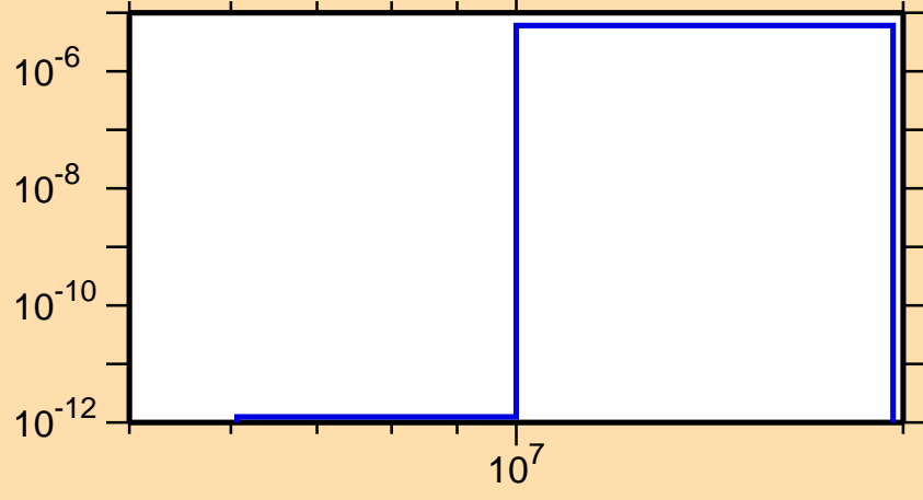
\sigma vs. E for ^{160}\text{Hf}(n,pd)
