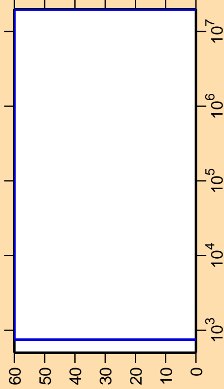
\Delta\sigma/\sigma vs. E for ^{160}\text{Hf}(n,p\alpha)
