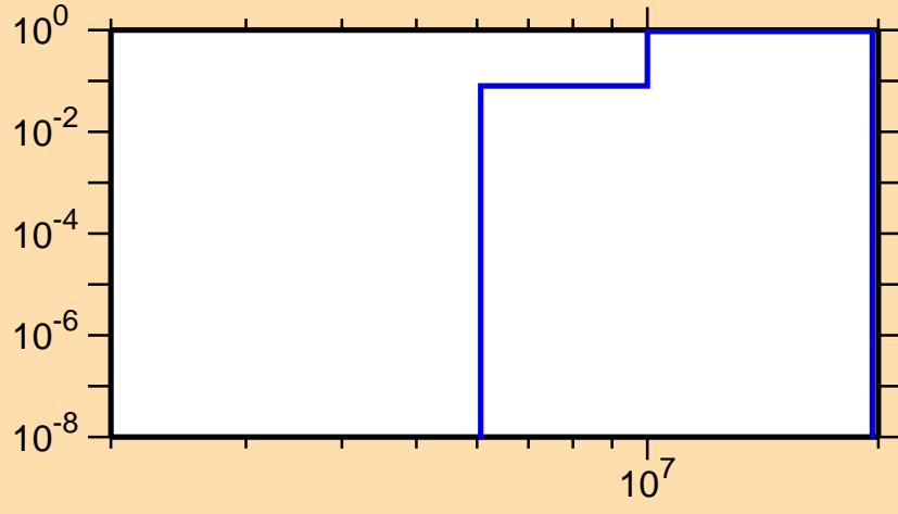
\sigma vs. E for ^{160}\text{Hf}(n,np)
